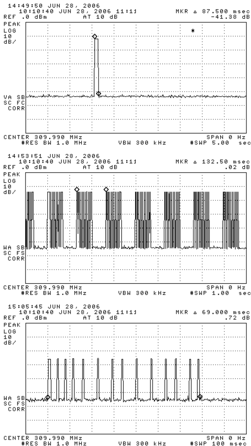
Figure 6.1(a). Transmissions modulation characteristics: (top) single transmission, (center) expanded period, (bottom) expanded word.
