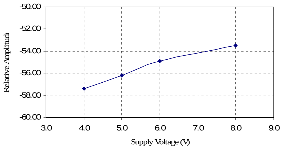
Figure 6.5. Relative emission at 310.0 MHz vs. supply voltage (pulsed emission).
