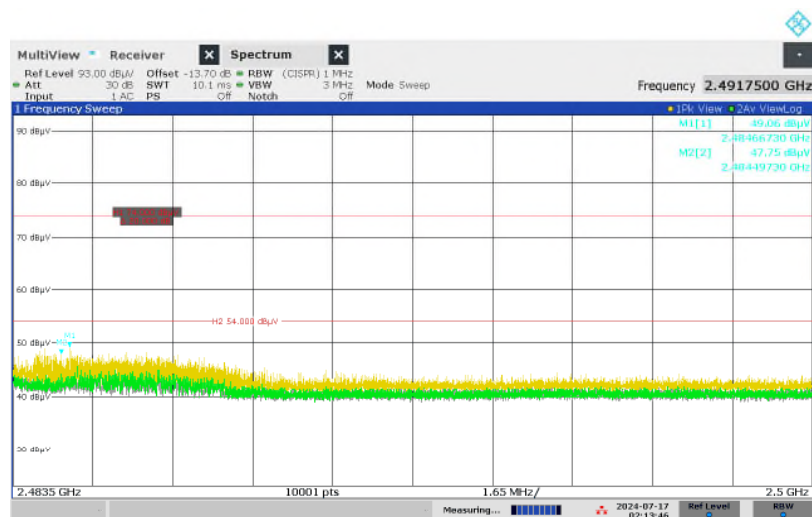
Figure 36: Restricted-band Band-edge, Spectral Diagram, BLE, 2480MHz, Horizontal Antenna Orientation, 2Mbps
