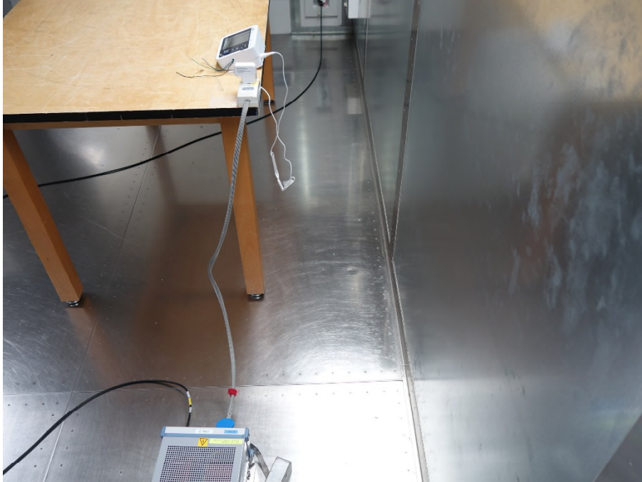
Photograph 9: Set-up for AC Power Line Conducted Emission, Rear View
