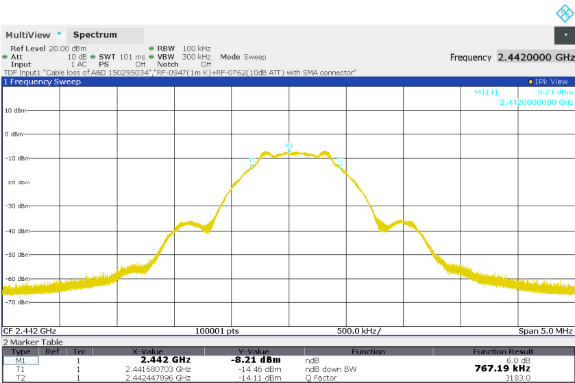
Figure 3: 6dB Bandwidth, BLE, Mode M (2442MHz), 1Mbps
