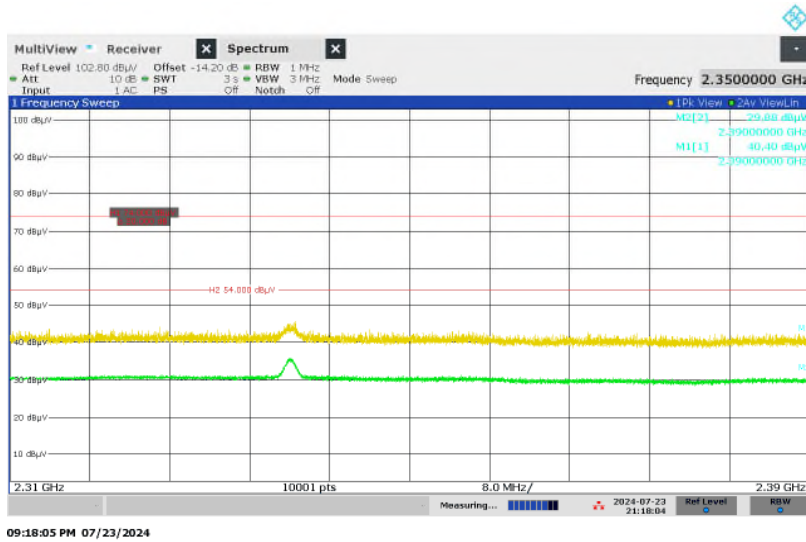
Figure 31: Restricted-band Band-edge, Spectral Diagram, BLE, 2402MHz, Vertical Antenna Orientation, 1Mbps
