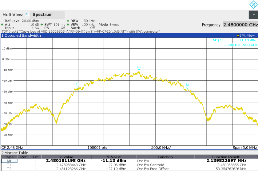
Figure 13: 99% Bandwidth, BLE, Mode H (2480MHz), 2Mbps
