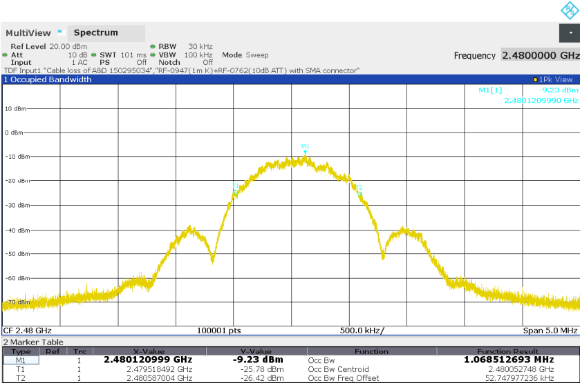
Figure 10: 99% Bandwidth, BLE, Mode H (2480MHz), 1Mbps
