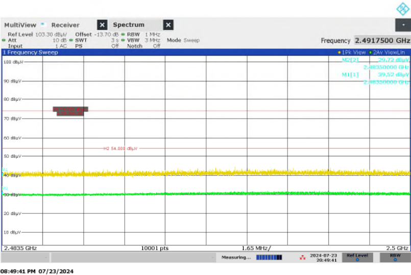
Figure 33: Restricted-band Band-edge, Spectral Diagram, BLE, 2480MHz, Vertical Antenna Orientation, 1Mbps
