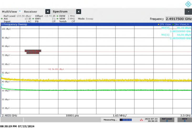
Figure 37: Restricted-band Band-edge, Spectral Diagram, BLE, 2480MHz, Vertical Antenna Orientation, 2Mbps
