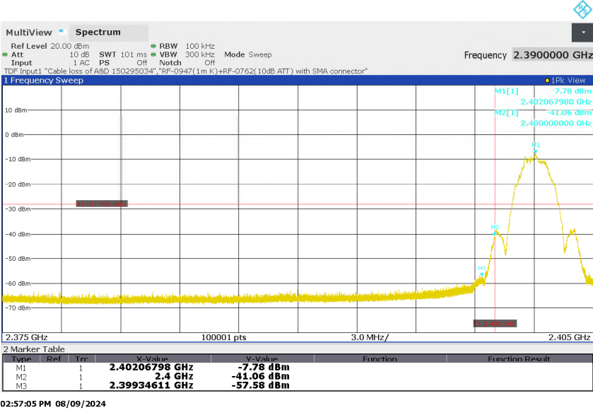
Figure 22: Authorized-band band-edge, BLE, Mode L (2402MHz), 2Mbps
