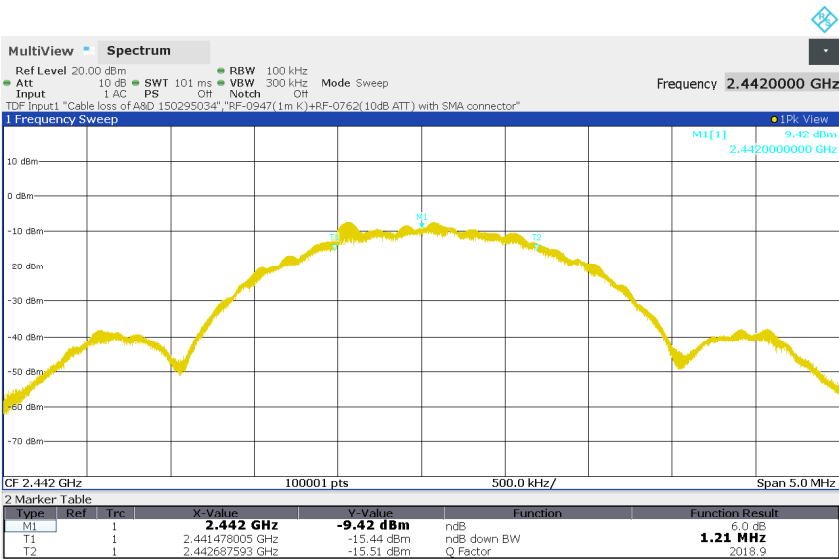
Figure 6: 6dB Bandwidth, BLE, Mode M (2442MHz), 2Mbps
