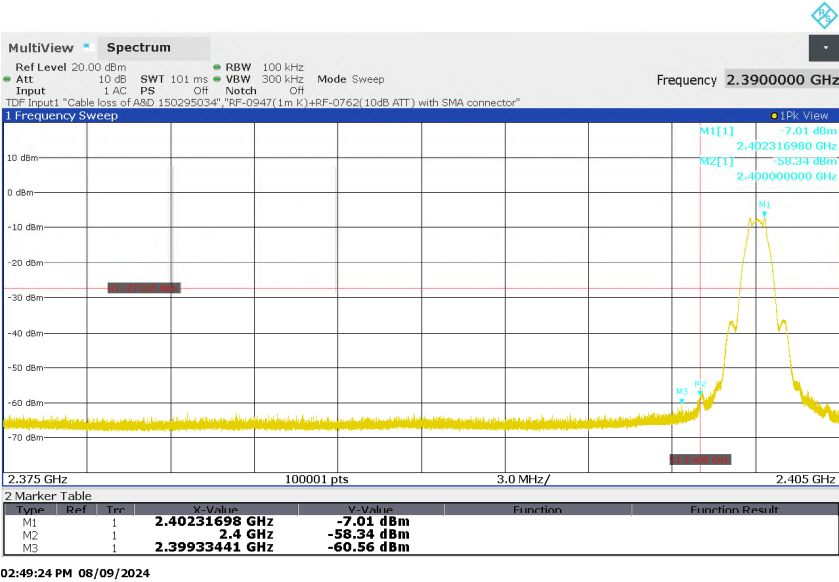
Figure 17: Authorized-band band-edge, BLE, Mode L (2402MHz), 1Mbps
