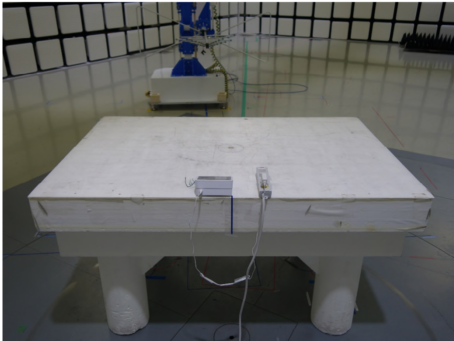
Photograph 5: Set-up for Radiated Spurious Emission below 1GHz, Rear View
