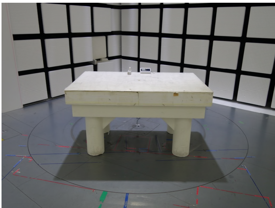
Photograph 2: Set-up for Radiated Spurious Emission below 30MHz, Front View
