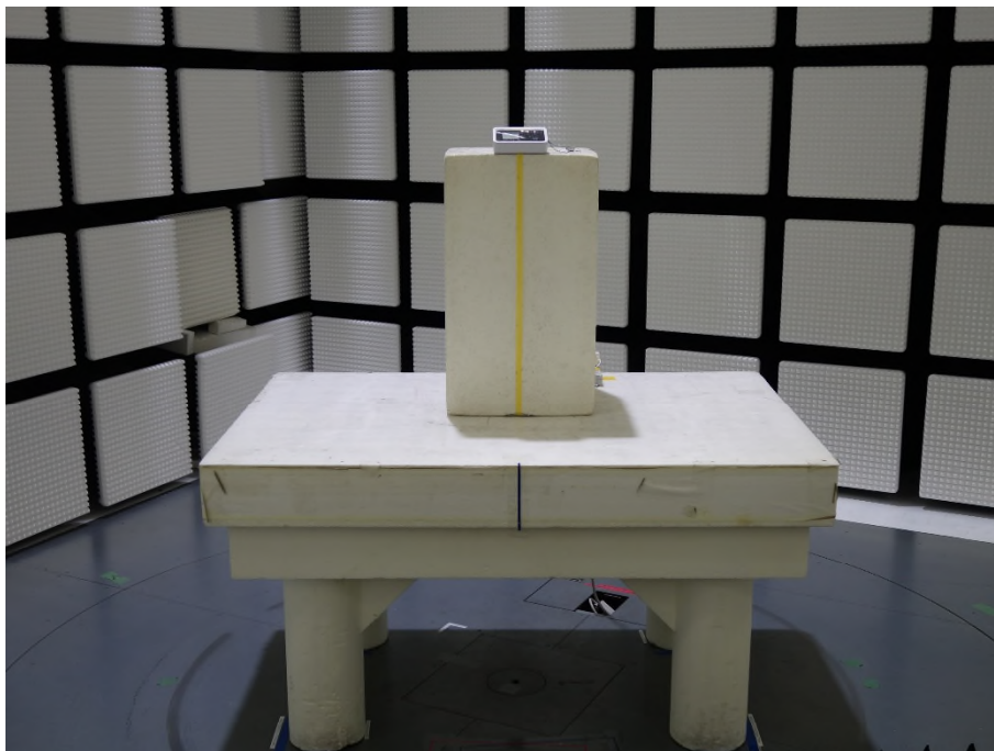
Photograph 6: Set-up for Radiated Spurious Emission above 1GHz, Front View
