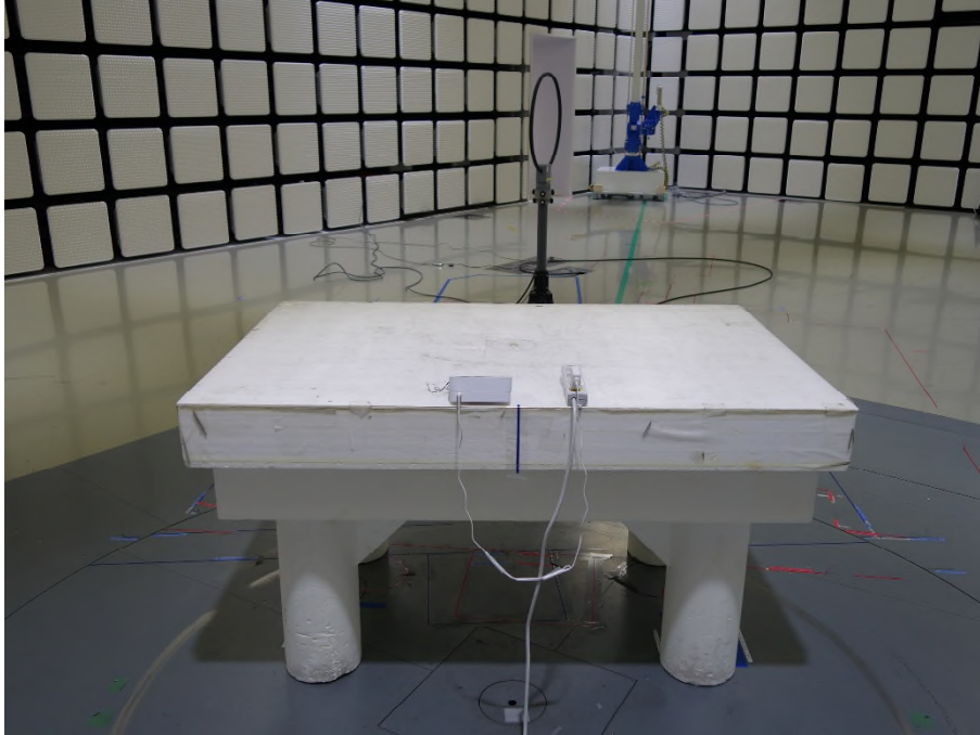
Photograph 3: Set-up for Radiated Spurious Emission below 30MHz, Rear View
