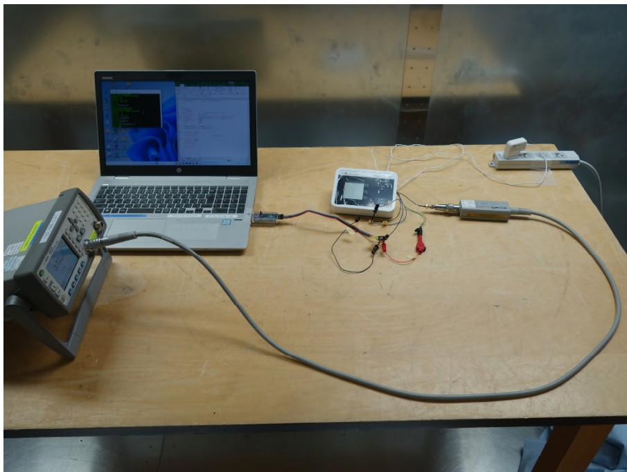
Photograph 1: Set-up for Antenna Port Conducted Emission of Transmitter
