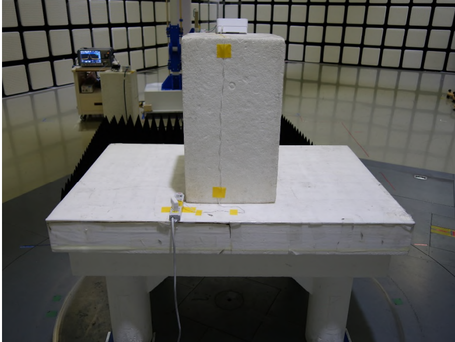
Photograph 7: Set-up for Radiated Spurious Emission above 1GHz, Rear View
