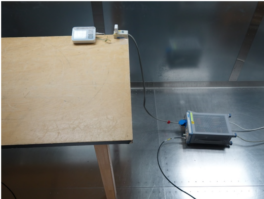
Photograph 8: Set-up for AC Power Line Conducted Emission, Front View
