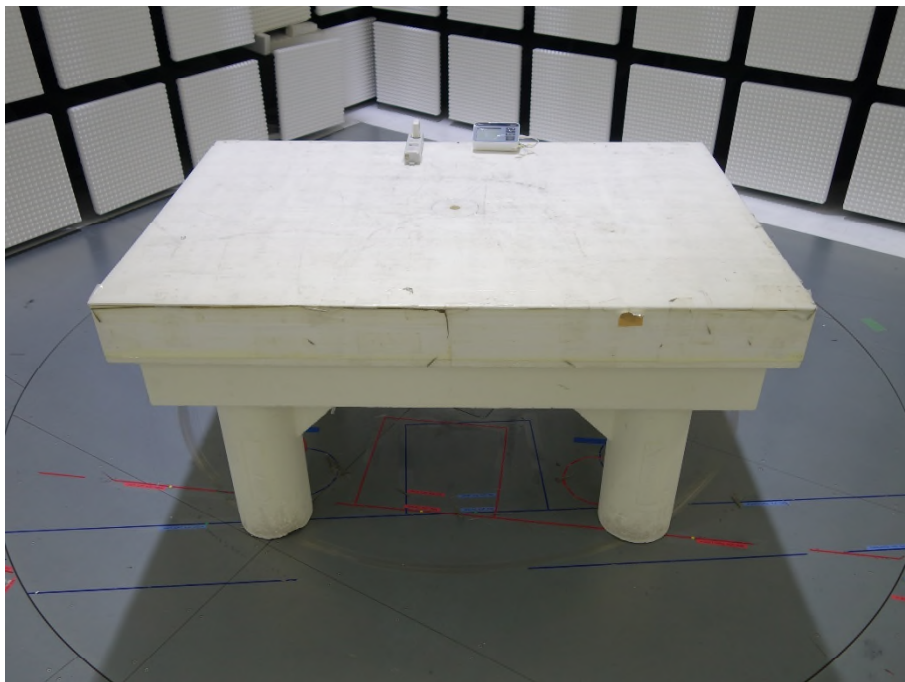
Photograph 4: Set-up for Radiated Spurious Emission below 1GHz, Front View
