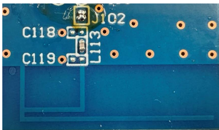
RF circuit
