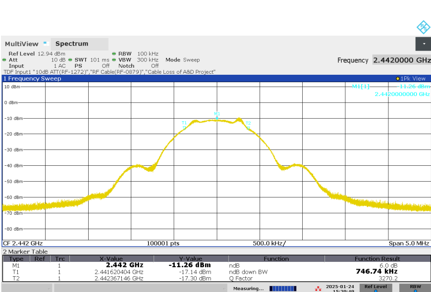
Figure 3: 6dB Bandwidth, BLE, Mode M (2442MHz), 1Mbps
