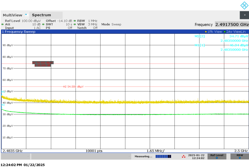
Figure 36: Restricted-band Band-edge, Spectral Diagram, Horizontal Antenna Orientation, BLE, Mode H (2480MHz), 2Mbps
