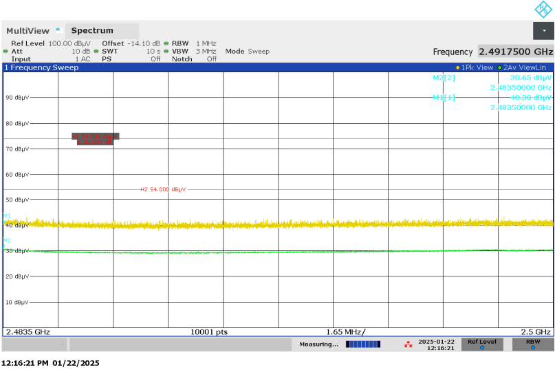
Figure 32: Restricted-band Band-edge, Spectral Diagram, Horizontal Antenna Orientation, BLE, Mode H (2480MHz), 1Mbps
