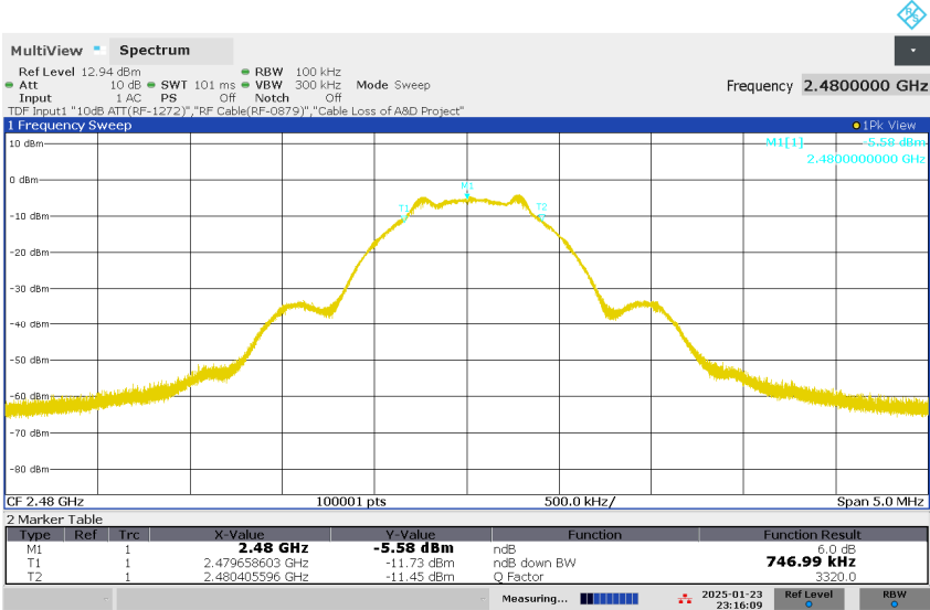
Figure 4: 6dB Bandwidth, BLE, Mode H (2480MHz), 1Mbps
