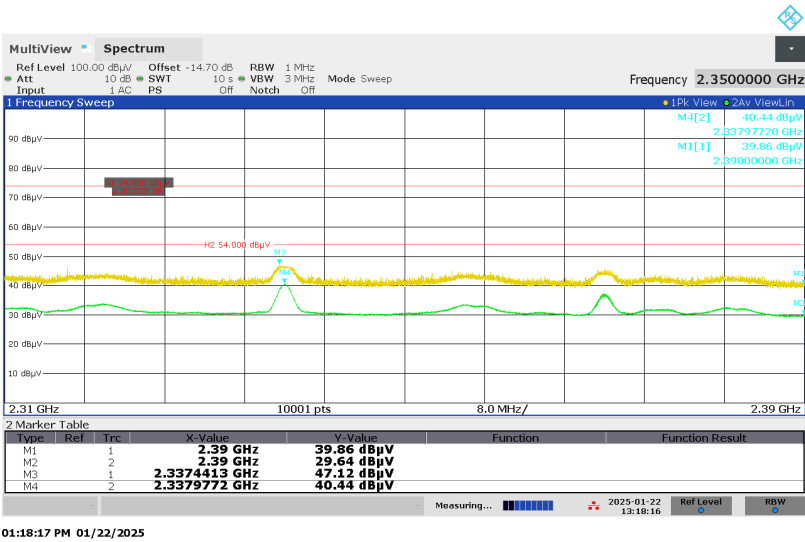
Figure 35: Restricted-band Band-edge, Spectral Diagram, Vertical Antenna Orientation, BLE, Mode L (2402MHz), 2Mbps
