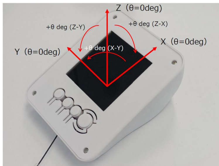
Definition of antenna measurement axis
