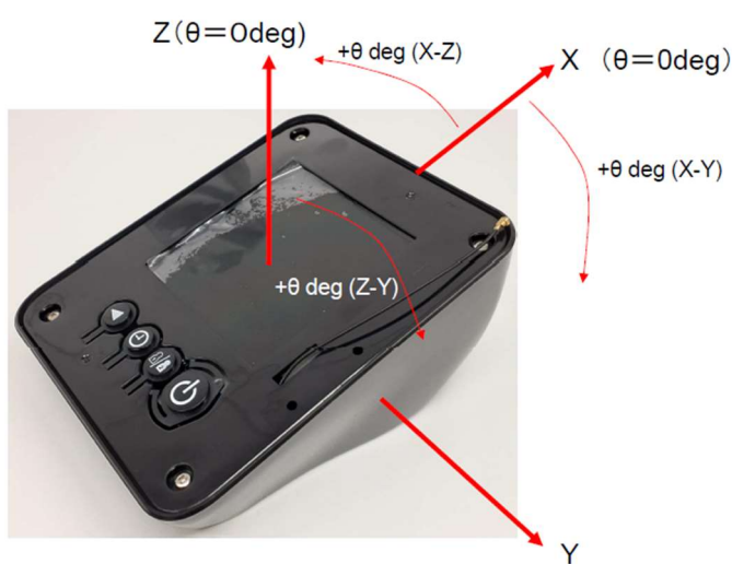
Antenna axis definition
