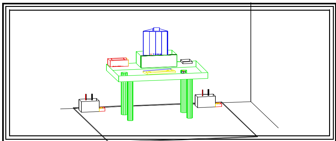
Fig. 10. System Setup. (See Attachment H - Test Photographs for actual system set-up.)
