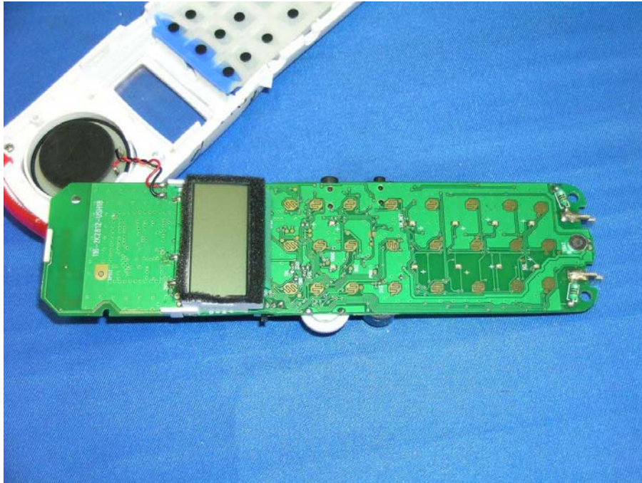
Handset Main PCB display side (View 1)
