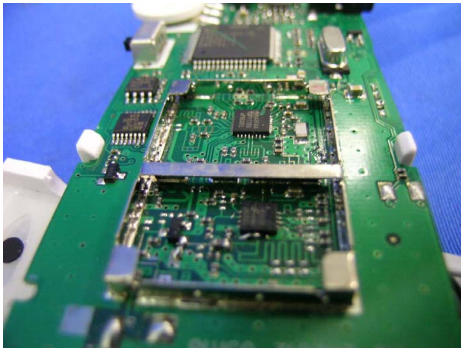
Handset Oscillator PCB comp side (View 2)
