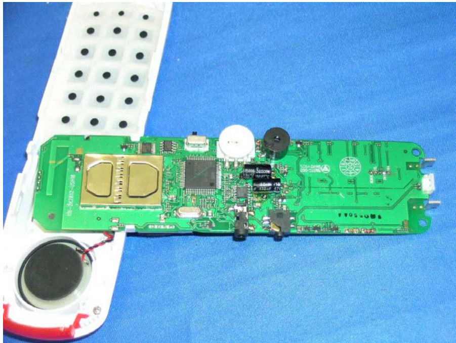
Handset Main PCB comp side
