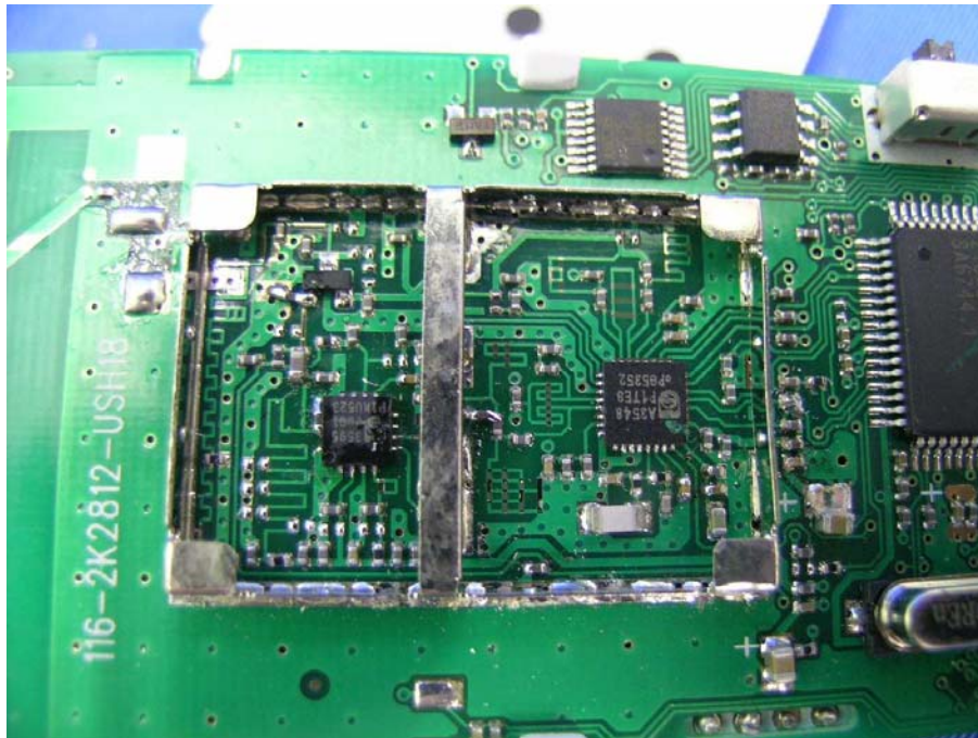
Handset Oscillator PCB comp side (View 1)
