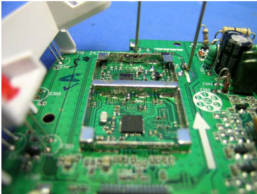
Base Unit Oscillator PCB comp side (View 3)
