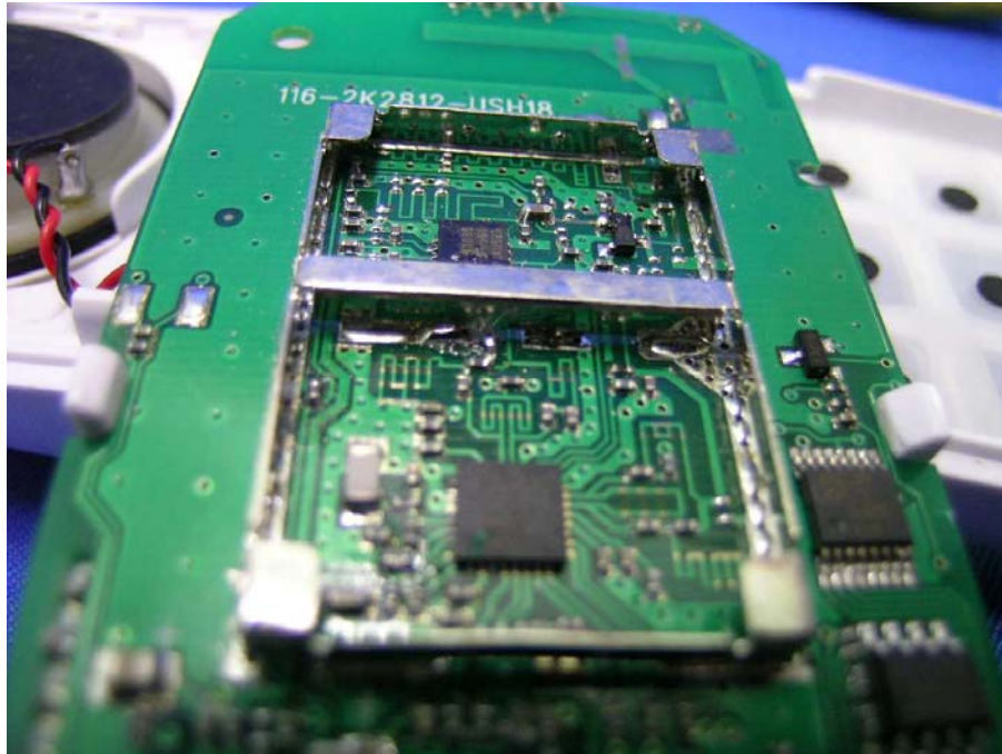
Handset Oscillator PCB comp side (View 3)
