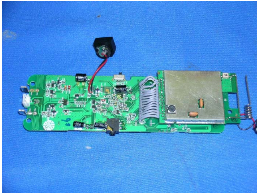
Handset Main PCB comp side (View 1)
