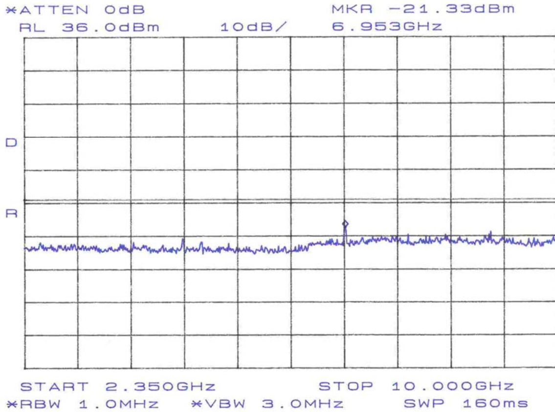
Figure 15. Emissions Mask, Channel 11
