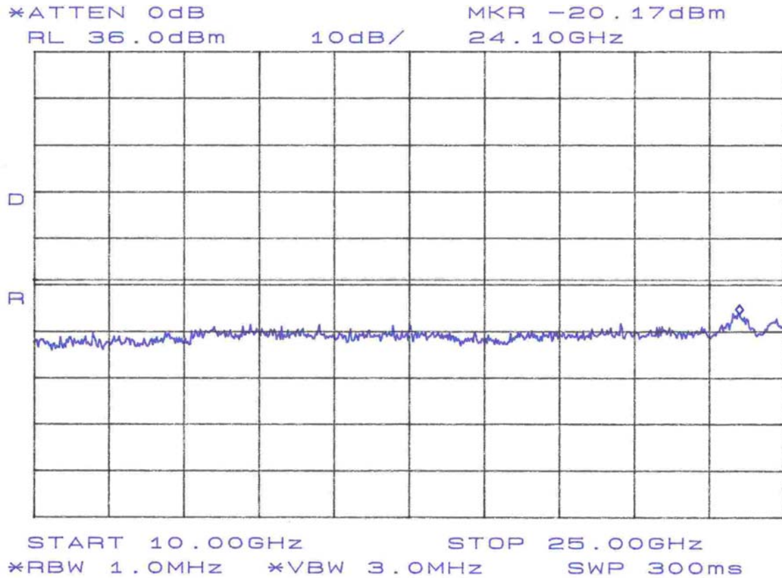
Figure 12. Emissions Mask, Channel 8
