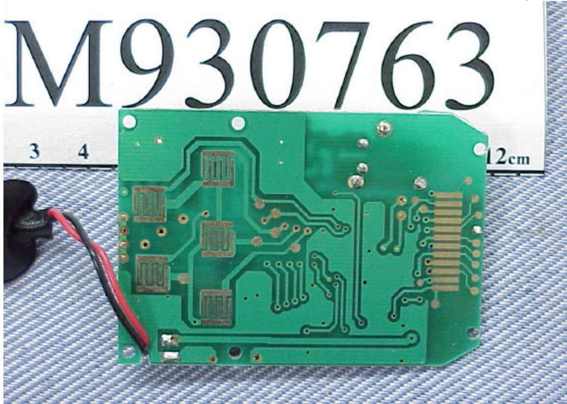
Photo 6 PCB View (Solder Side)
