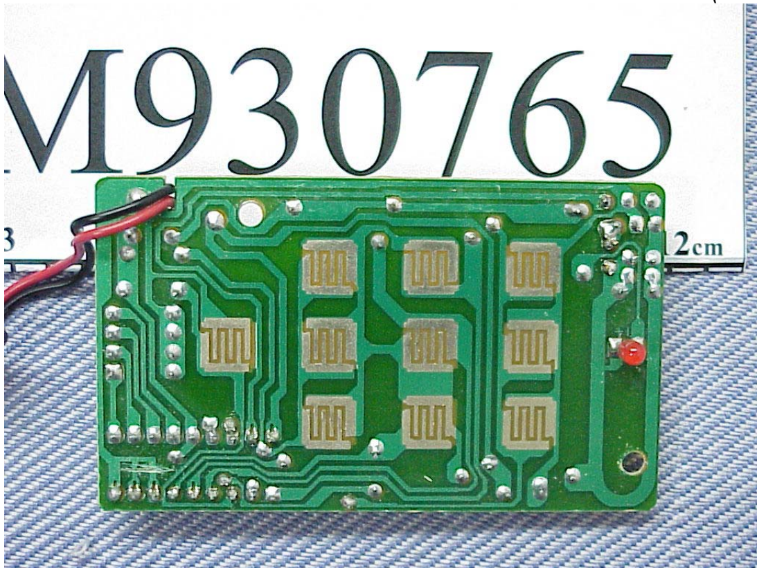
Photos 6 P. C. Board View (Solder Side)
