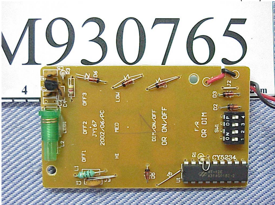
Photos 5 P. C. Board View (Component Side)
