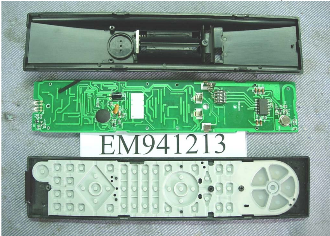
Photo 3 Internal View (Covers Removed)
