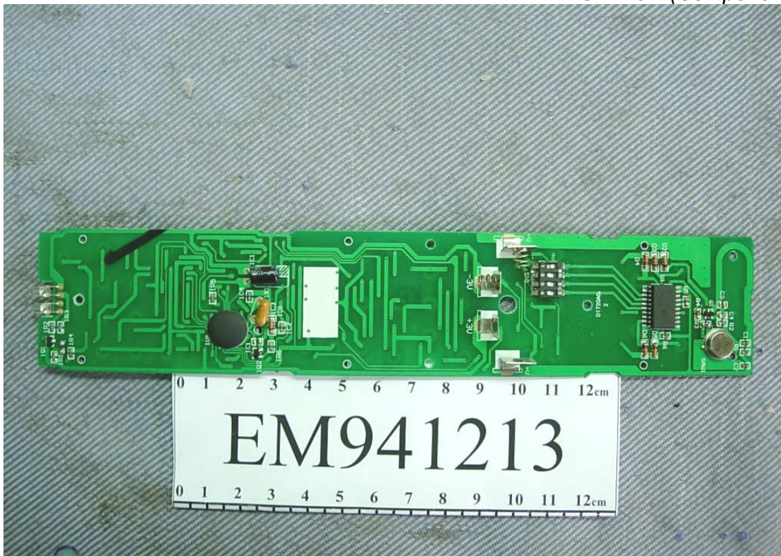
Photo 4 PCB View (Component Side)
