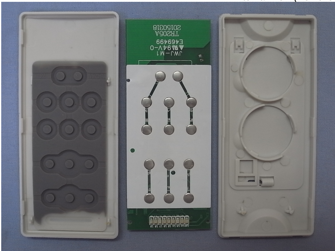
Photo 7 Internal View (Removed Cover)
