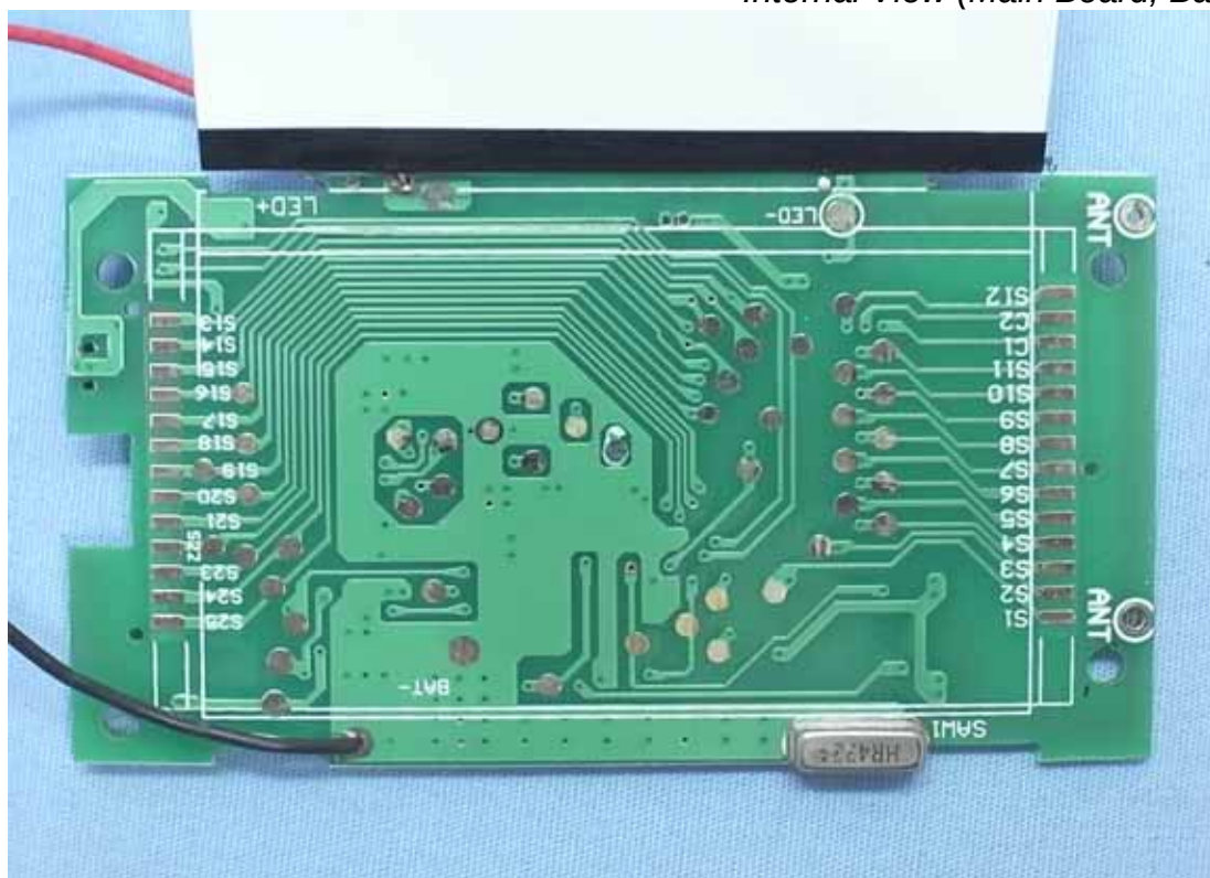
Photo 8 Internal View (Main Board, Back View)
