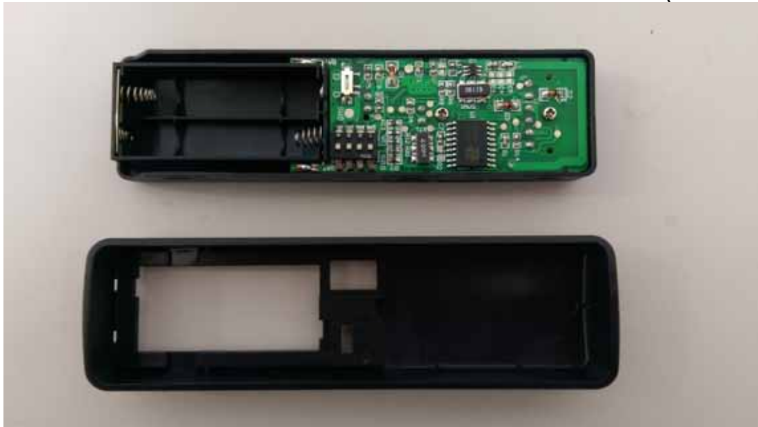
Photo 4 Internal View (Removed Cover)
