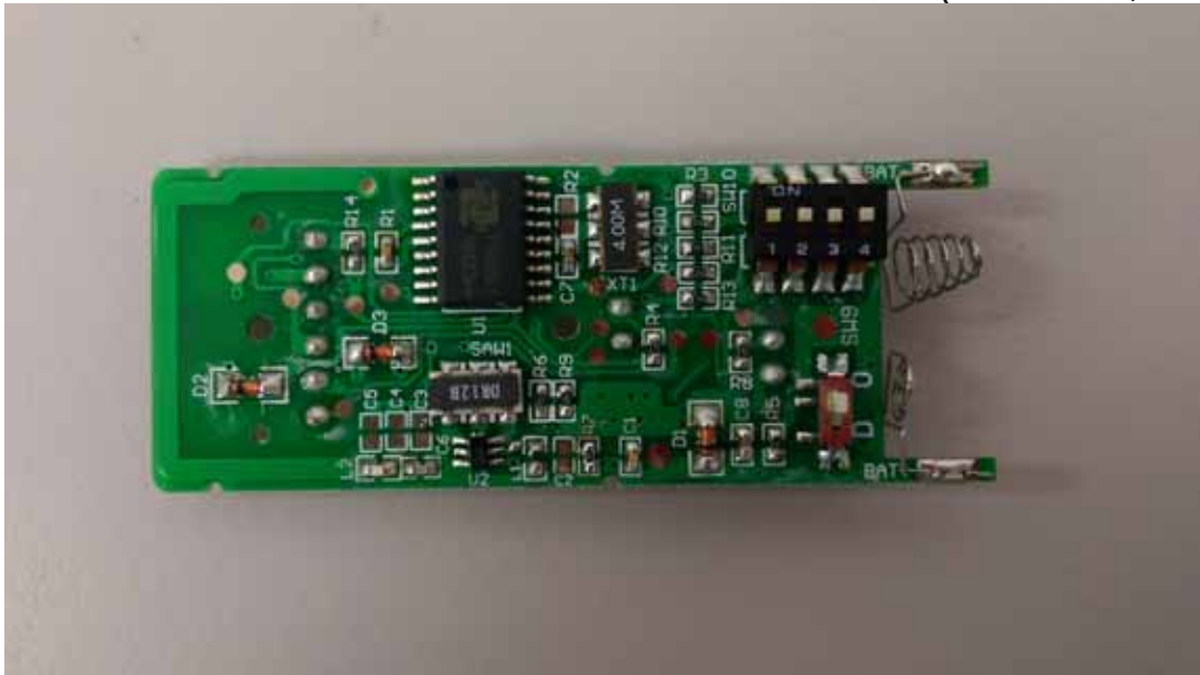
Photo 6 Internal View (Main Board, Front View)
