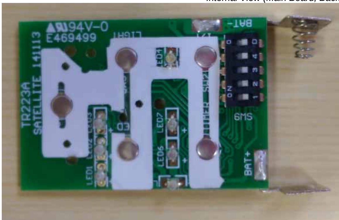
Photo 5 Internal View (Main Board, Back View)
