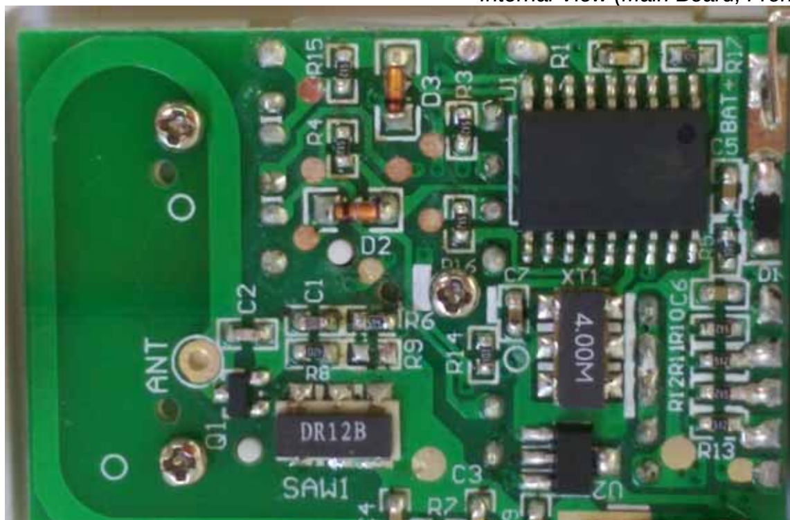
Photo 6 Internal View (Main Board, Front View)
