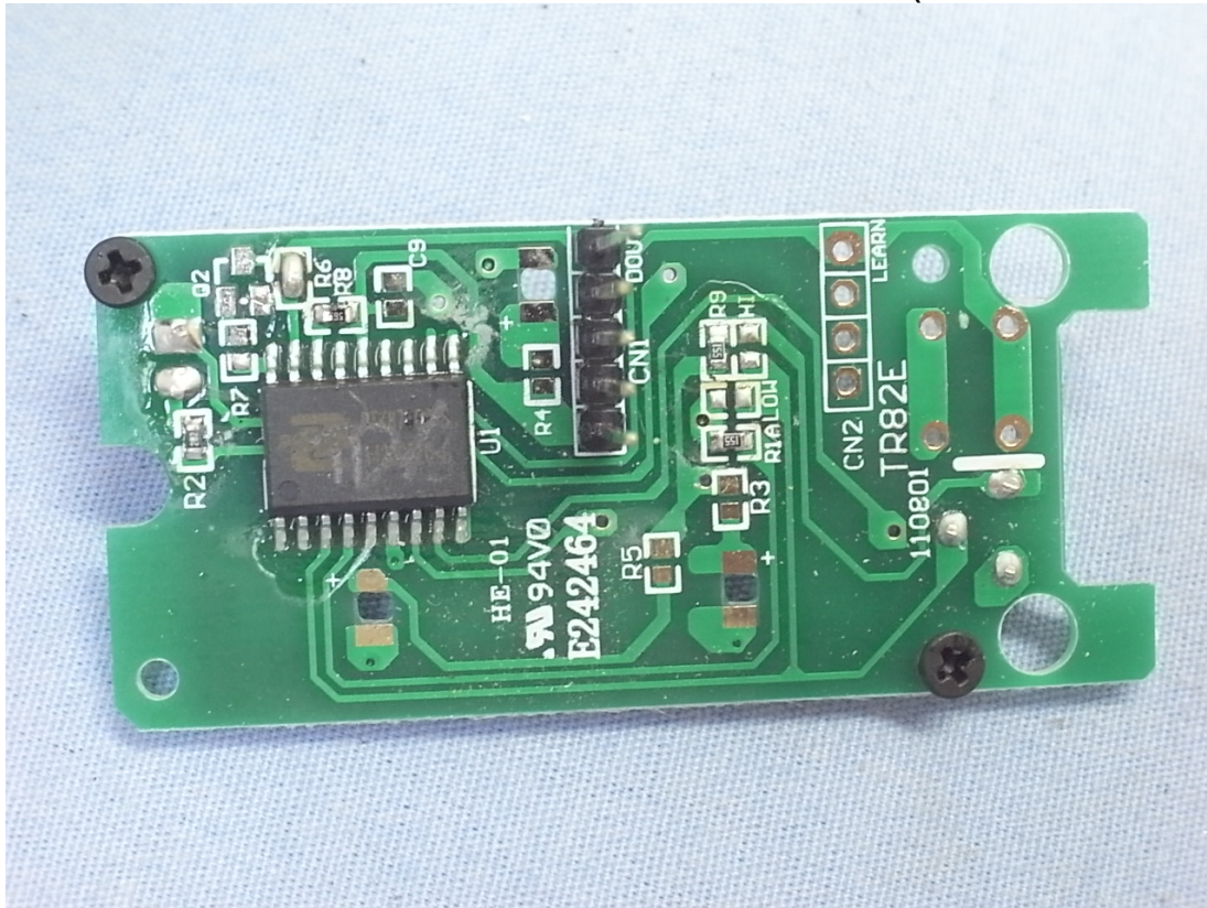
Photo 9 Internal View (Control Board, Front View)
