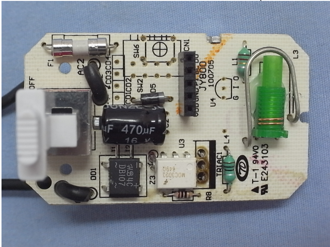
Photo 7 Internal View (Main Board, Front View)
