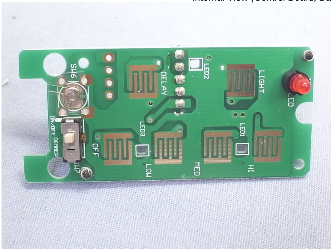
Photo 10 Internal View (Control Board, Back View)
