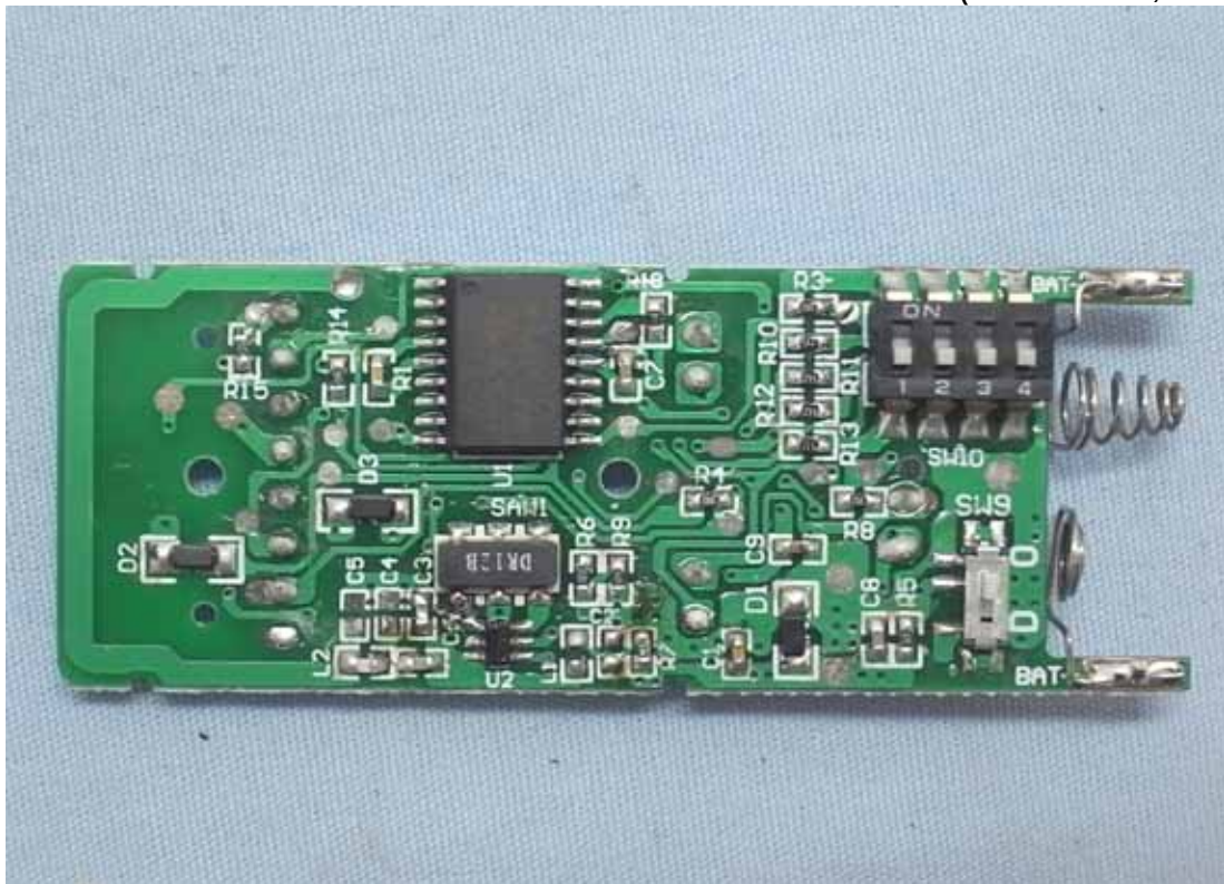
Photo 6 Internal View (Main Board, Front View)
