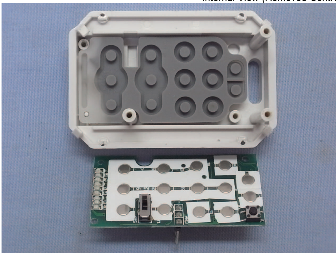
Photo 8 Internal View (Removed Control Board)
