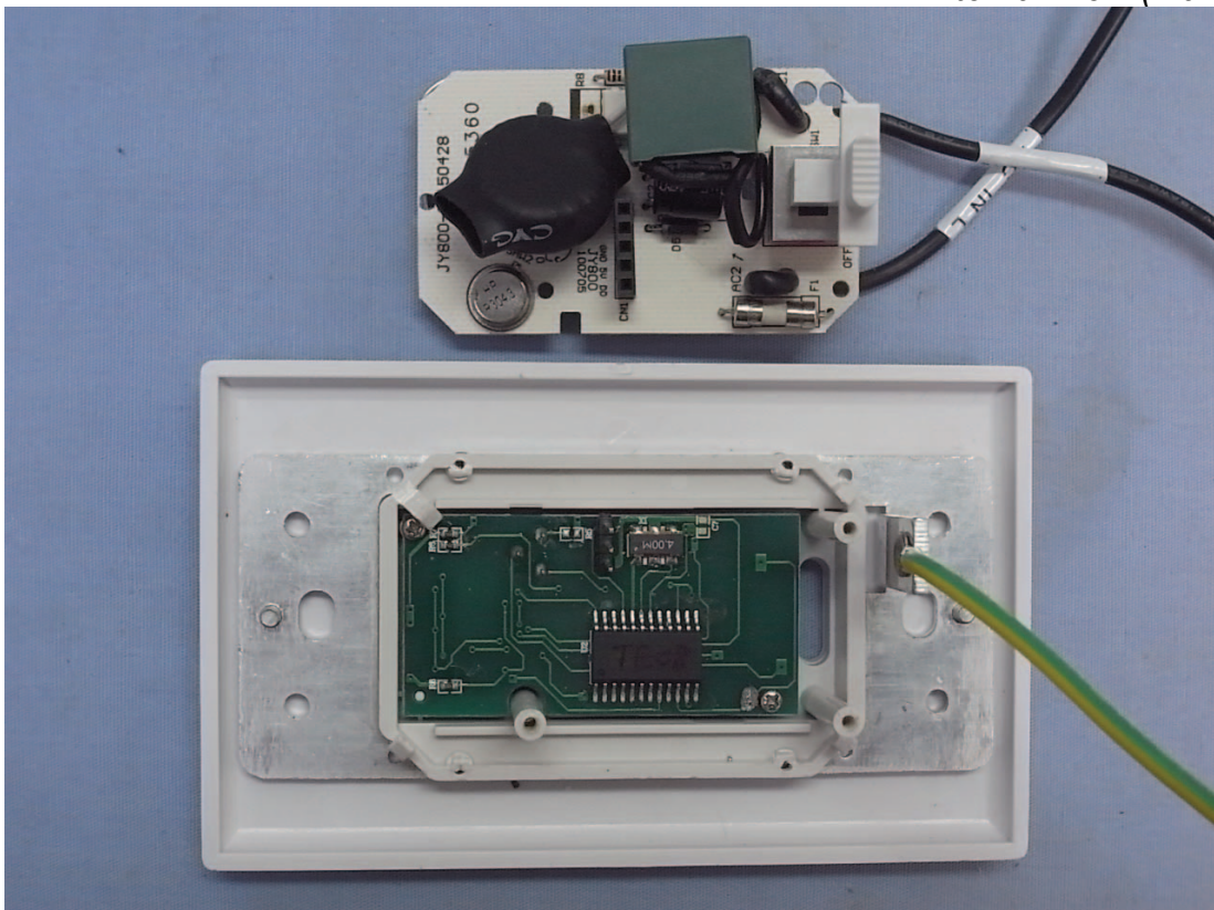
Photo 4 Internal View (Main Board)
