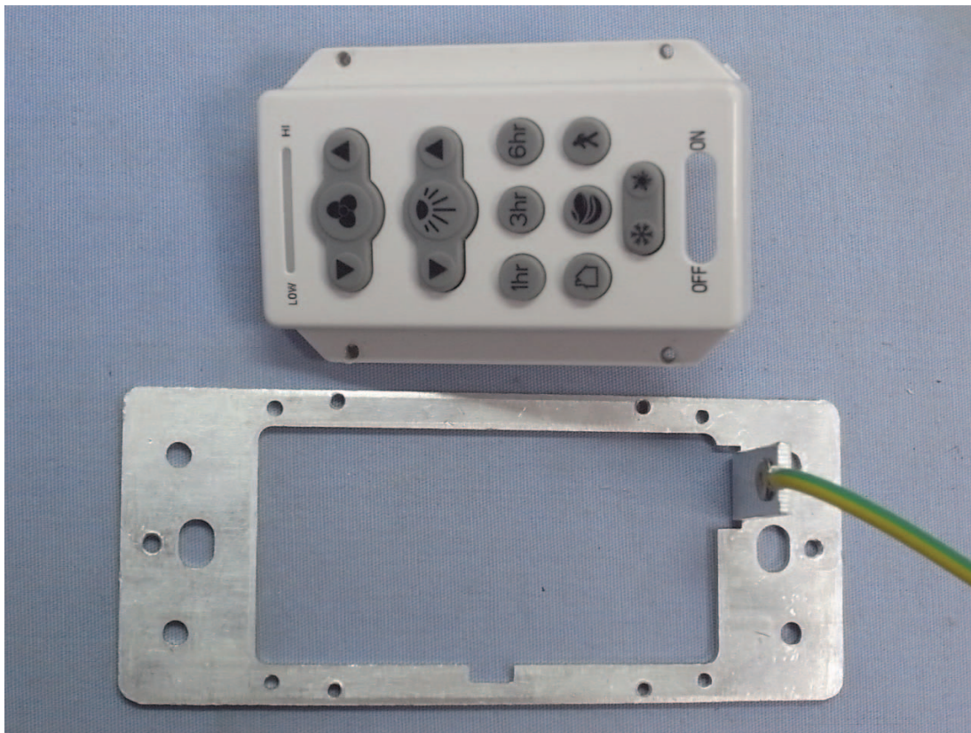
Photo 7 Internal View
