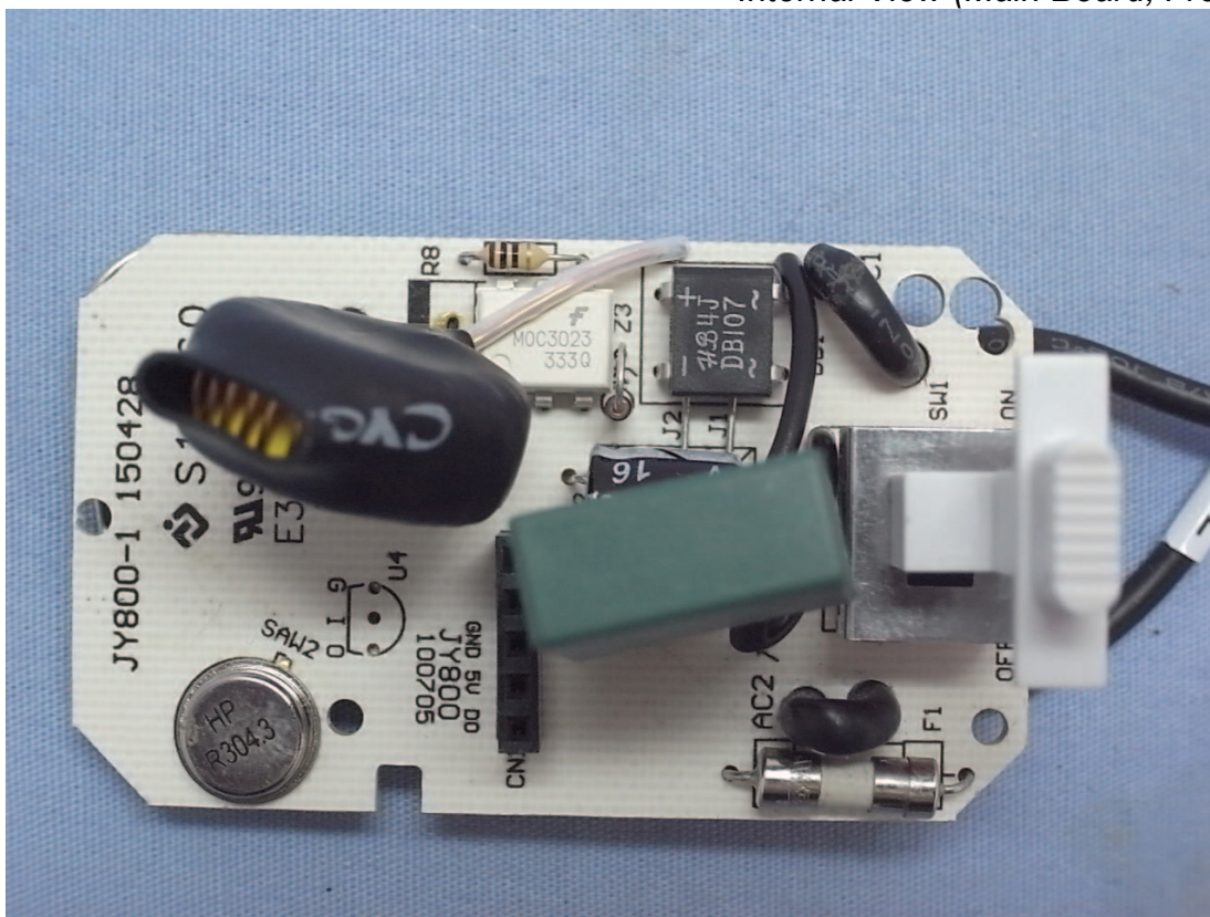
Photo 5 Internal View (Main Board, Front View)
