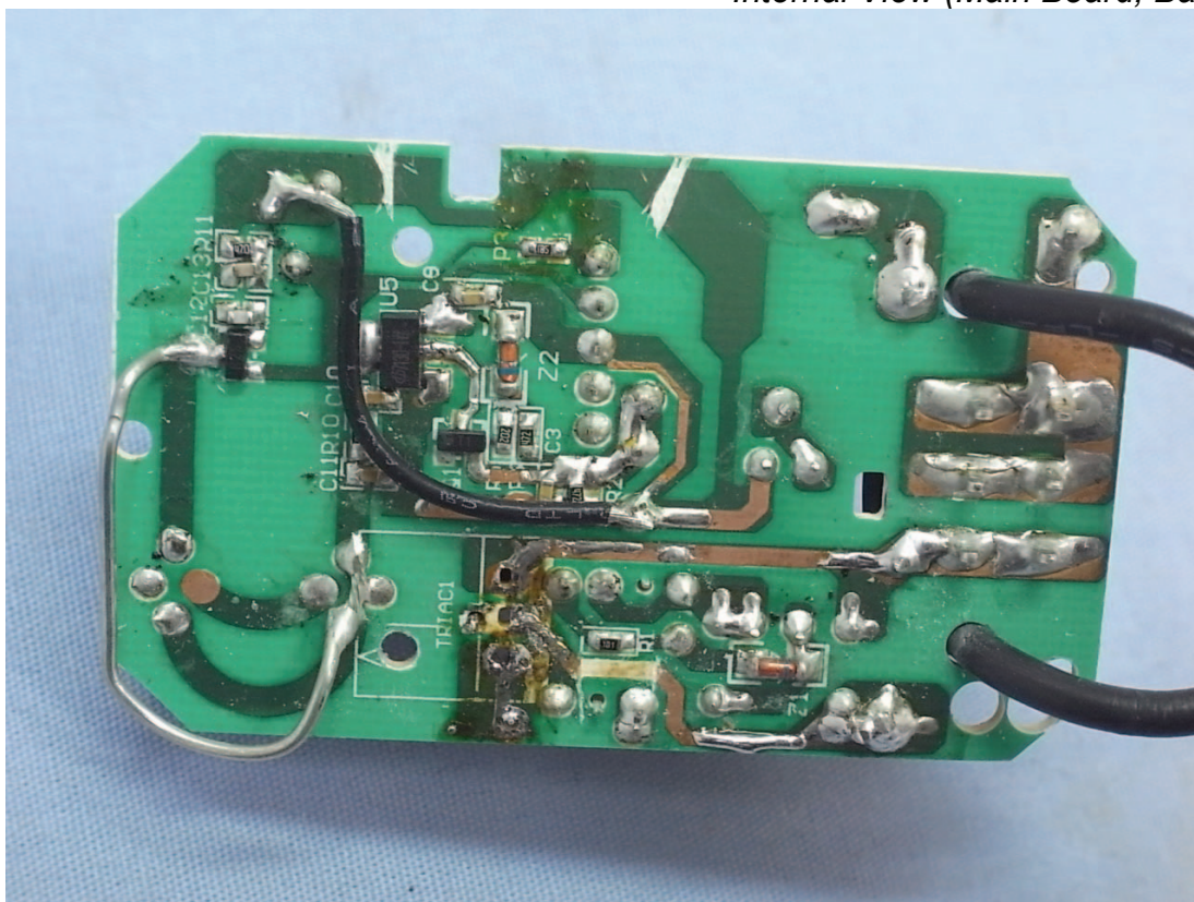
Photo 6 Internal View (Main Board, Back View)
