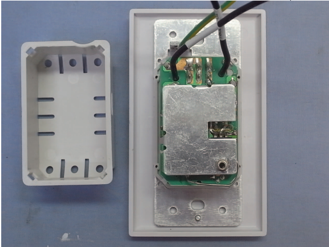
Photo 3 Internal View (Removed Cover)
