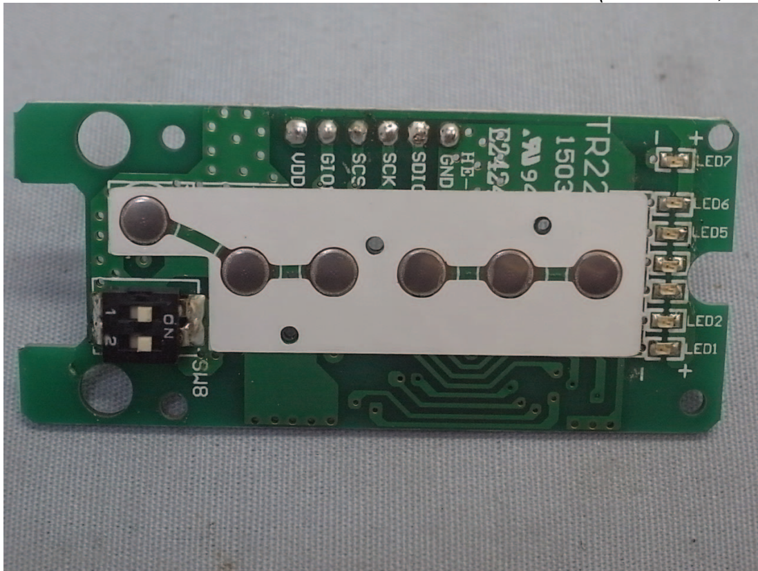
Photo 11 Internal View (Main Board, Back View)
