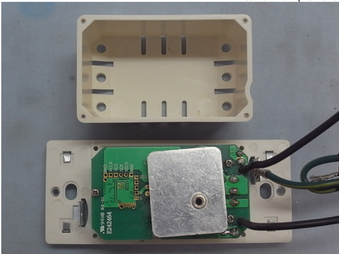
Photo 6 Internal View (Removed Cover)
