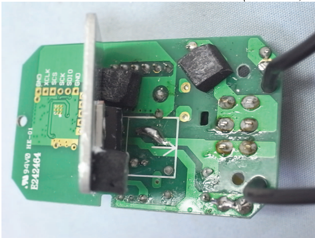
Photo 9 Internal View (Power Board, Back View)
