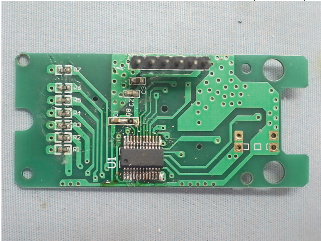
Photo 10 Internal View (Main Board, Front View)
