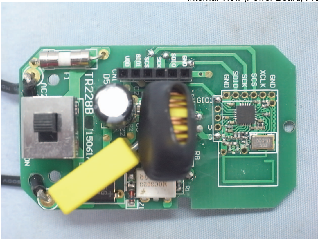
Photo 8 Internal View (Power Board, Front View)
