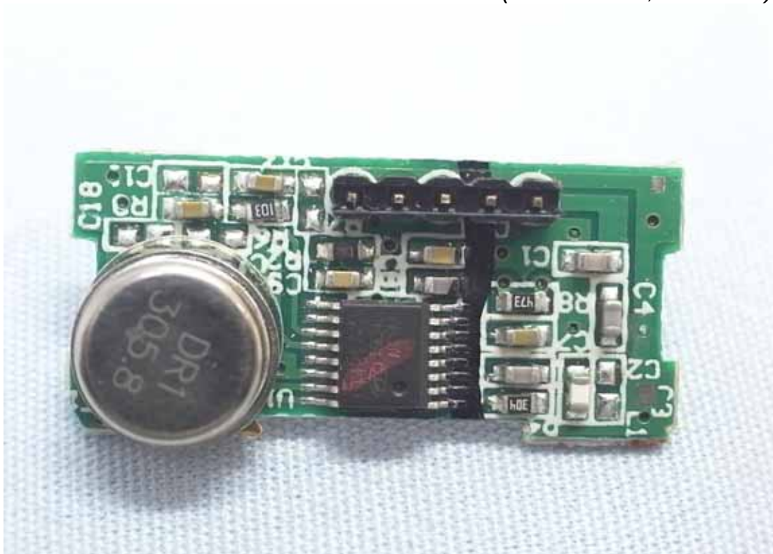
Figure 8 Internal View (Control Board, Back View)
