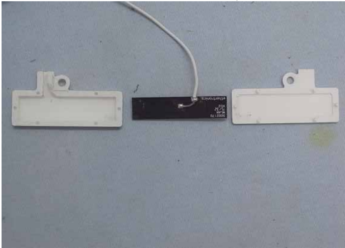
Figure 12 RF Antenna, Internal View Front & Back View
