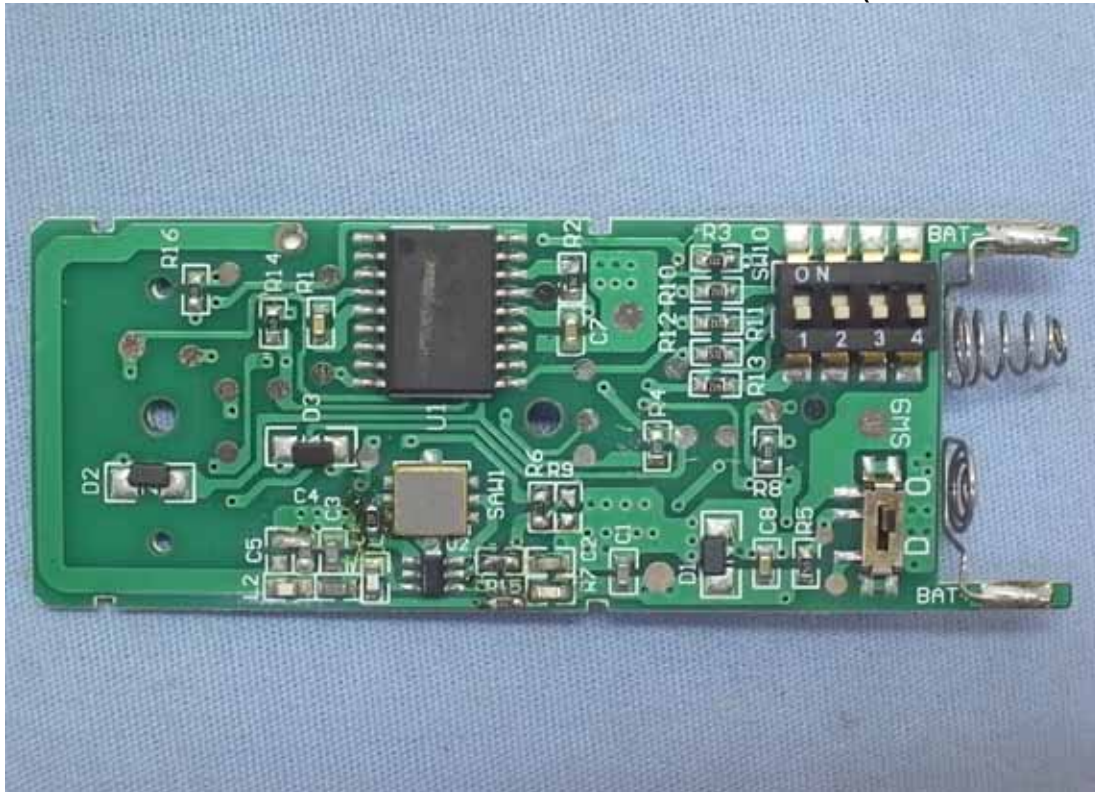
Photo 5 Internal View (Main Board, Front View)
