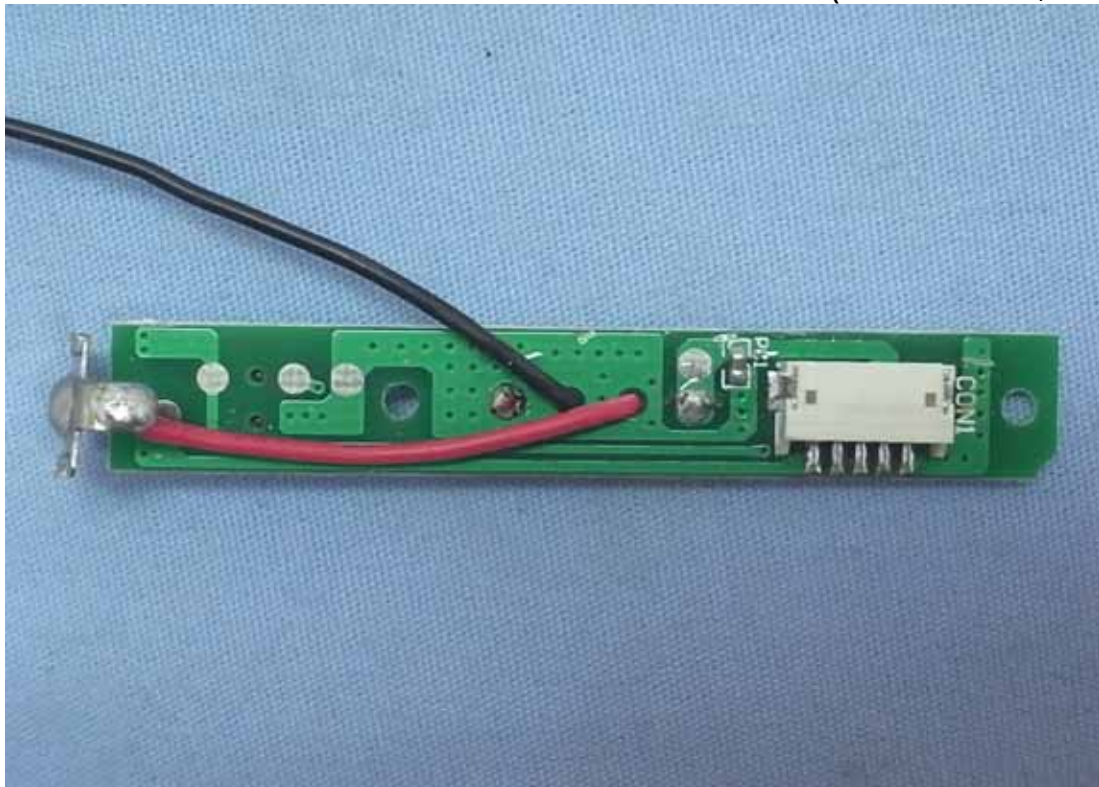
Photo 8 Internal View (Control Board, Back View)
