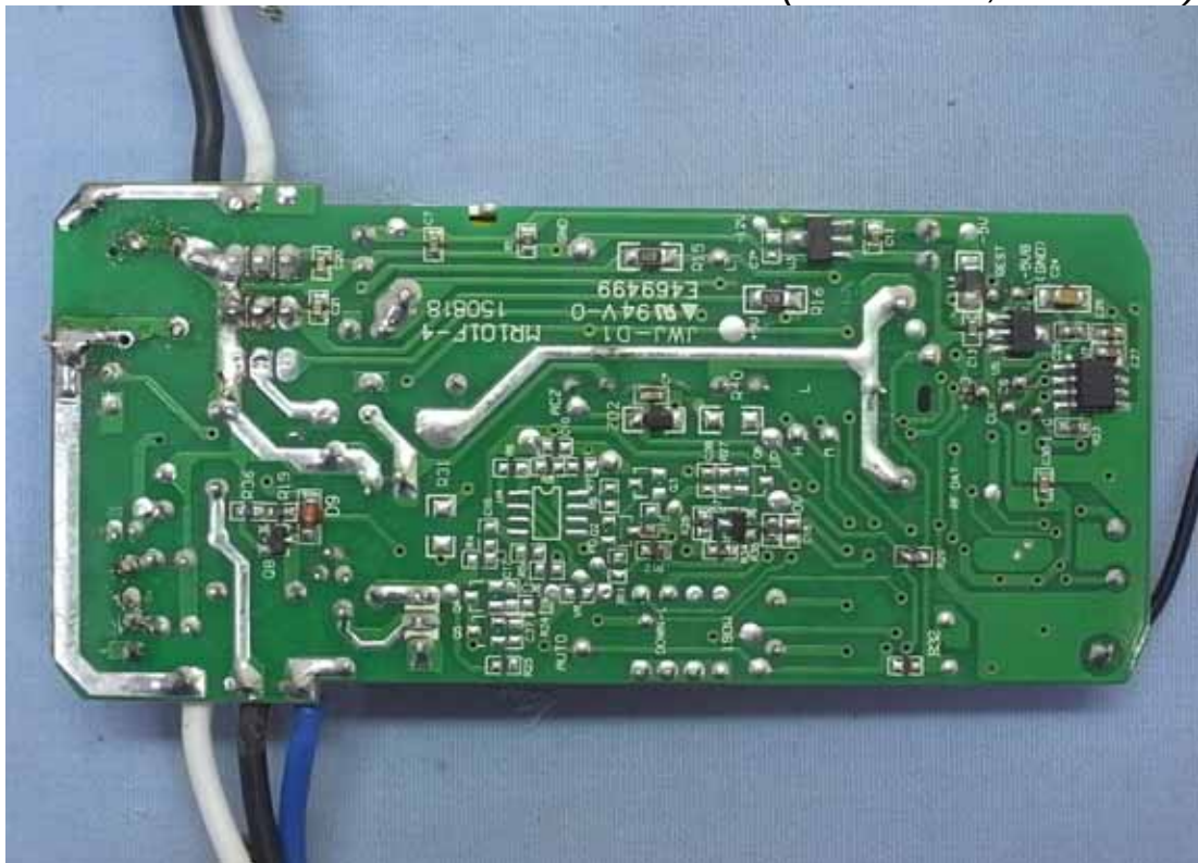
Figure 5 Internal View (Main Board, Back View)
