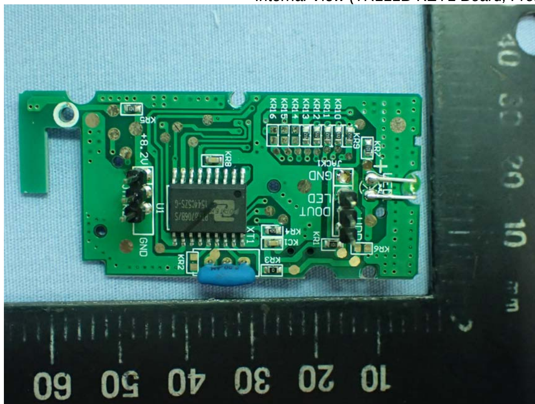
Photo 12 Internal View (TR111B-KEY1 Board, Back View)
