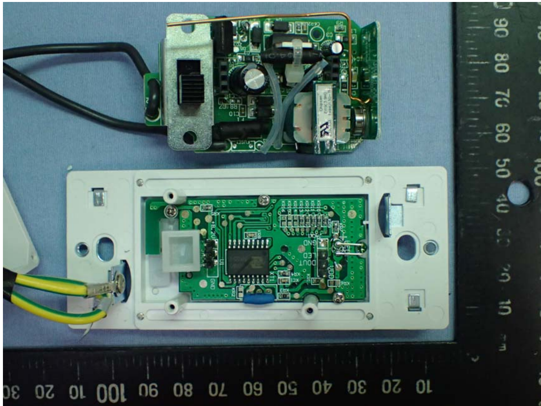
Photo 6 Internal View
