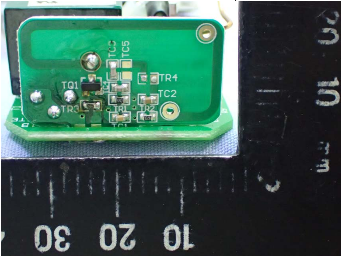
Photo 10 Internal View (TR111A-TX Board, Back View)
