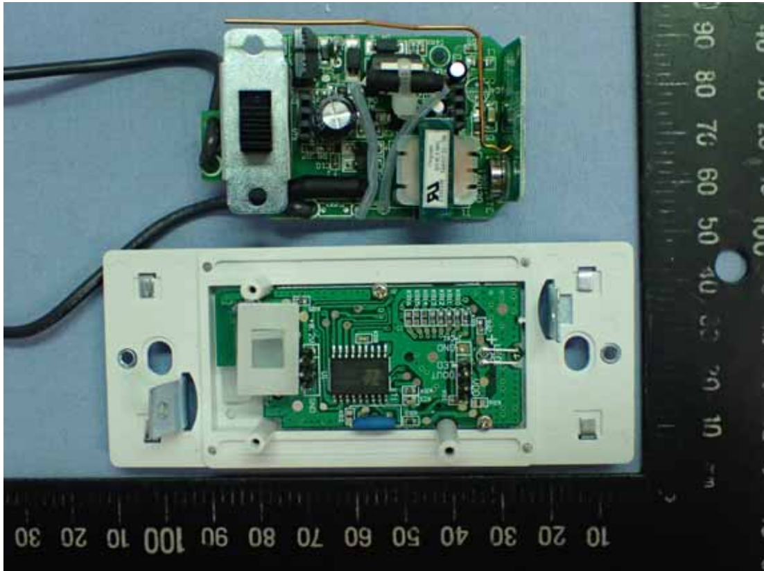
Photo 5 Internal View
