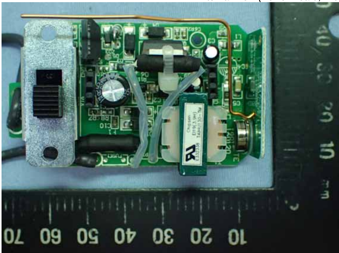
Photo 6 Internal View (Power Board, Front View)
