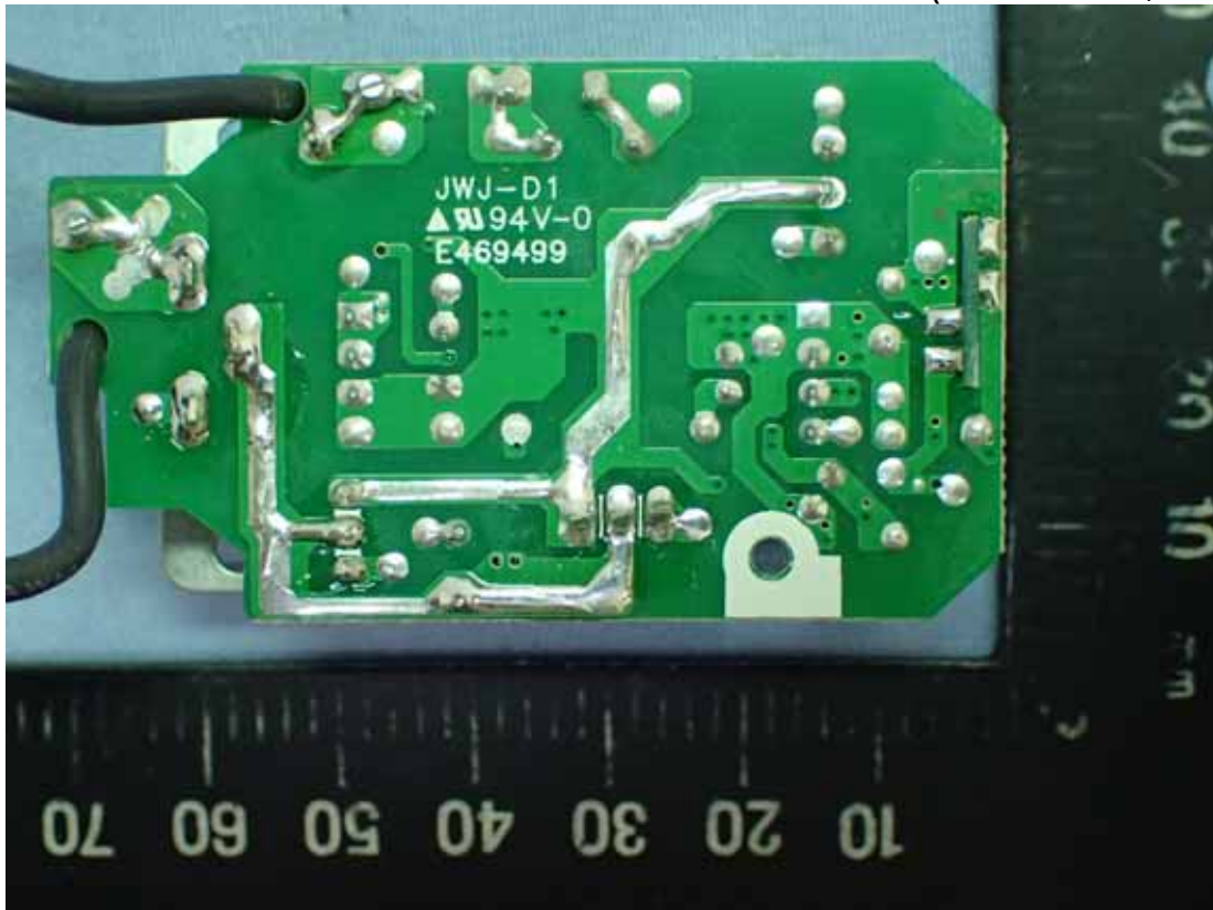
Photo 7 Internal View (Power Board, Back View)
