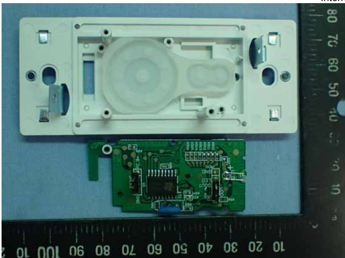
Photo 10 Internal View
