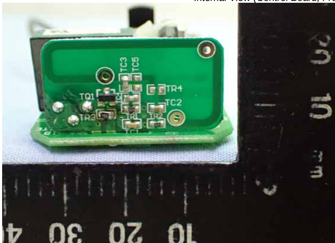
Photo 8 Internal View (Control Board, Front View)
