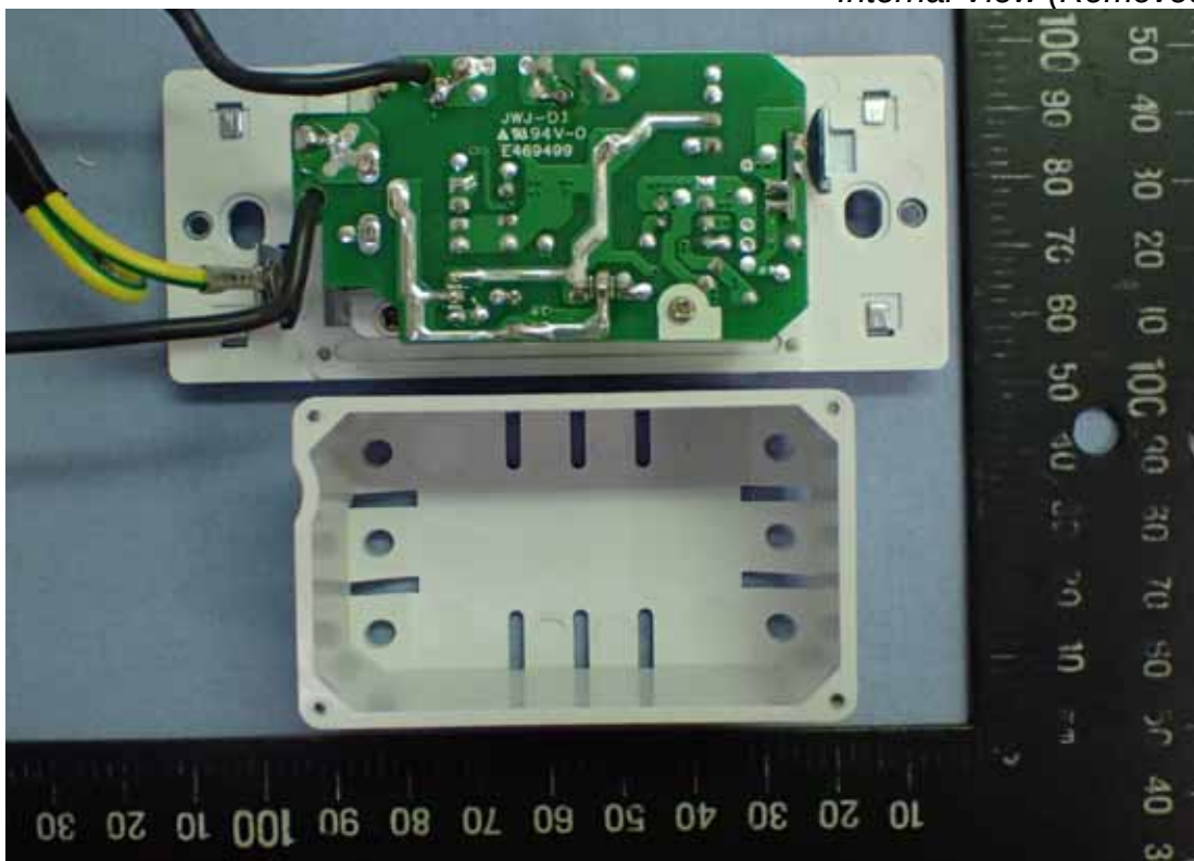
Photo 4 Internal View (Removed Cover)
