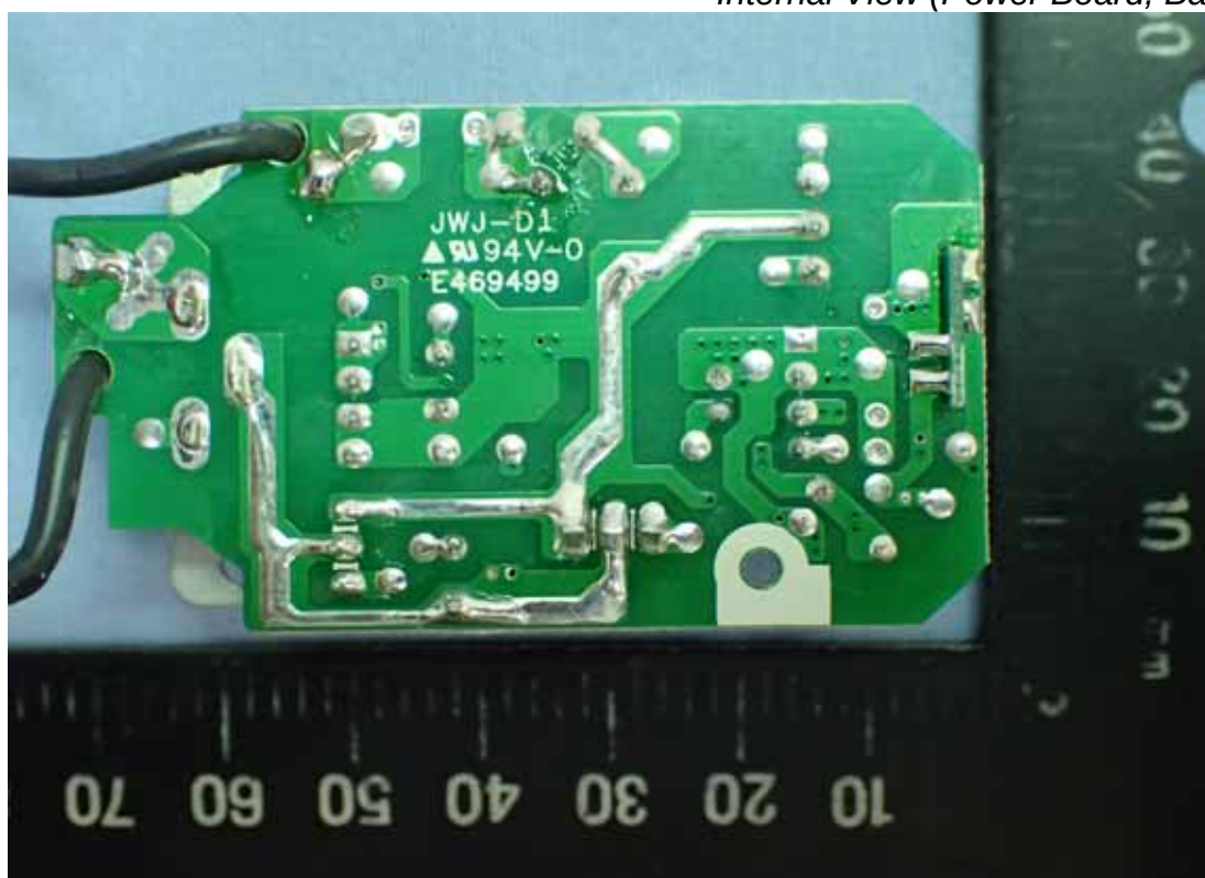
Photo 7 Internal View (Power Board, Back View)
