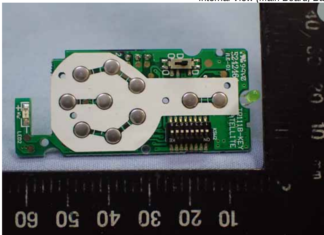
Photo 12 Internal View (Main Board, Back View)
