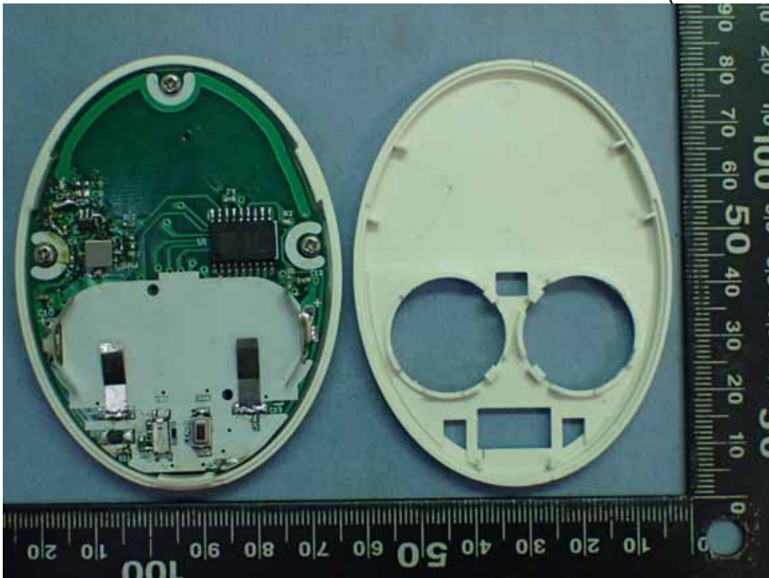
Photo 10 Internal View (Removed Main Board)
