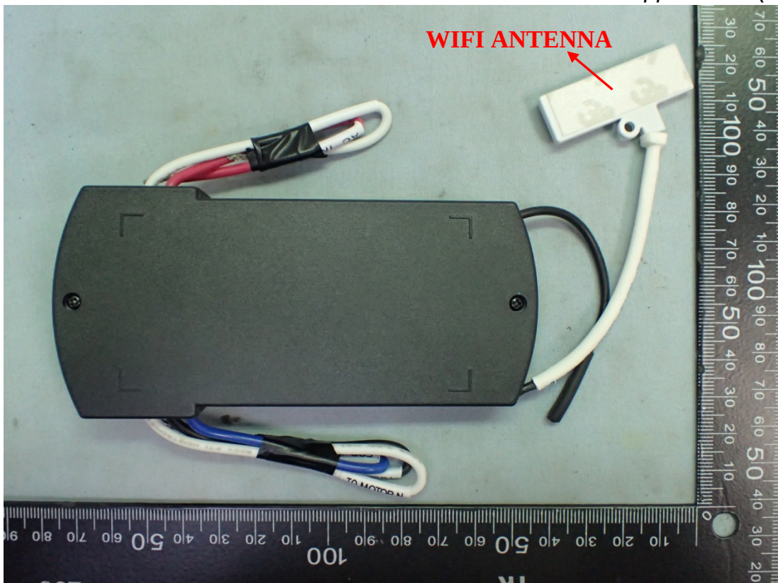
Figure 2 General Appearance (Side View)
