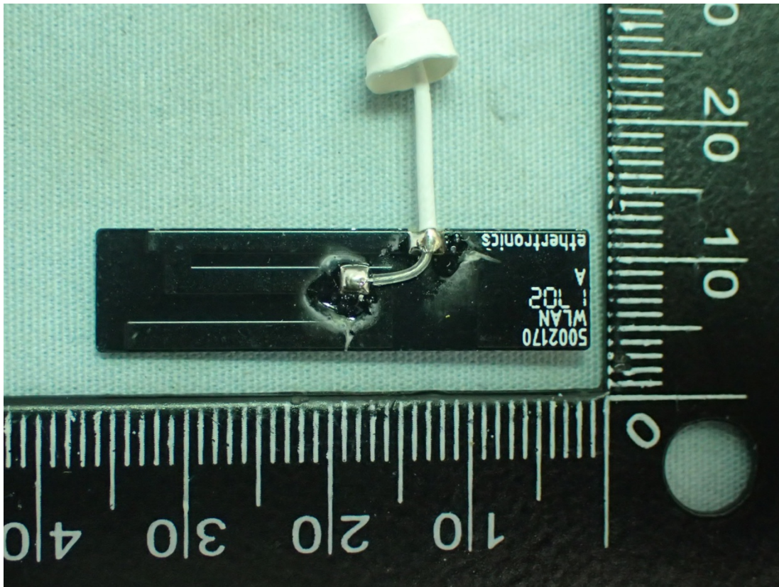
Figure 15 Internal View (WIFI Antenna (P/N: 5002170), Back View)
