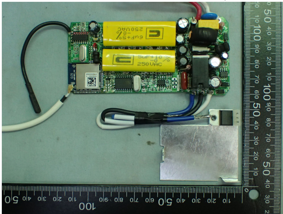
Figure 5 Internal View (Removed Metal Cover)
