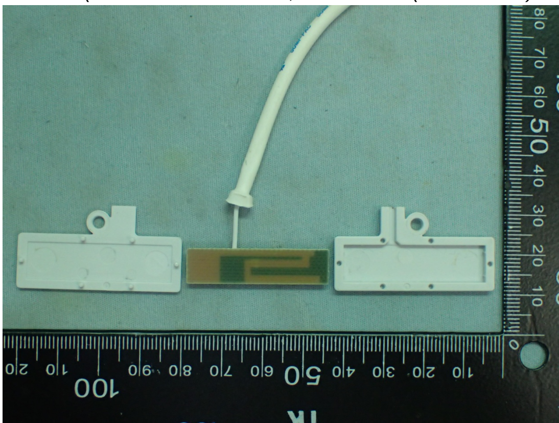
Figure 14 Internal View (Removed Antenna Cover, WIFI Antenna (P/N: 5002170)/Front View)
