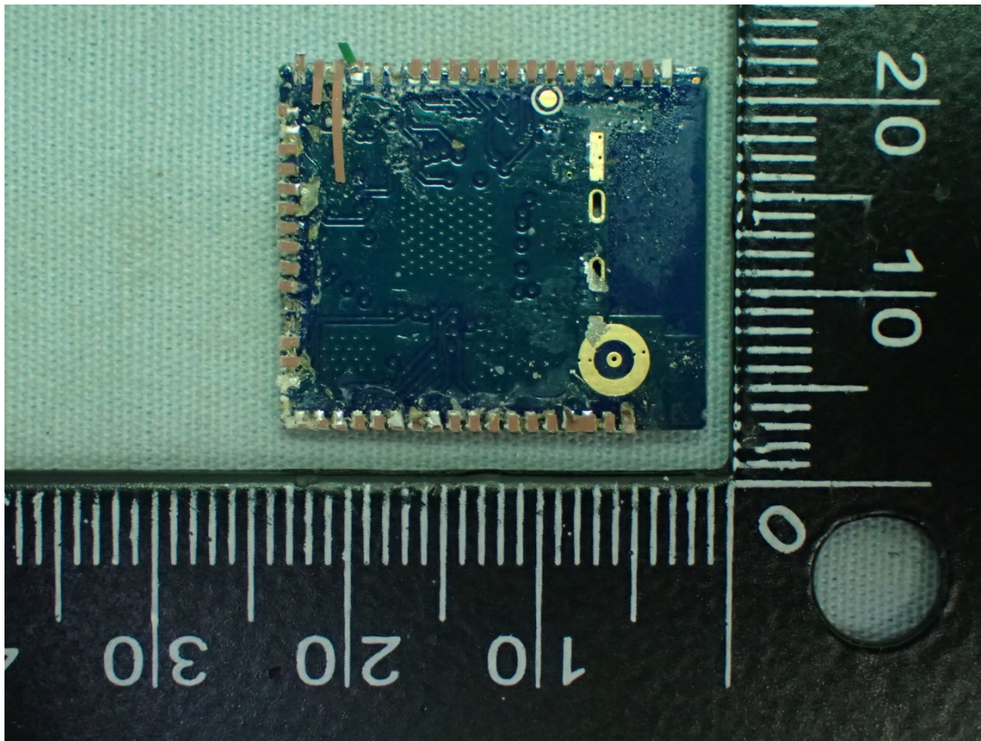
Figure 13 Internal View (WLAN Module, Back View)
