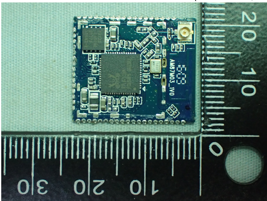
Figure 12 Internal View (WLAN Module, Front View)
