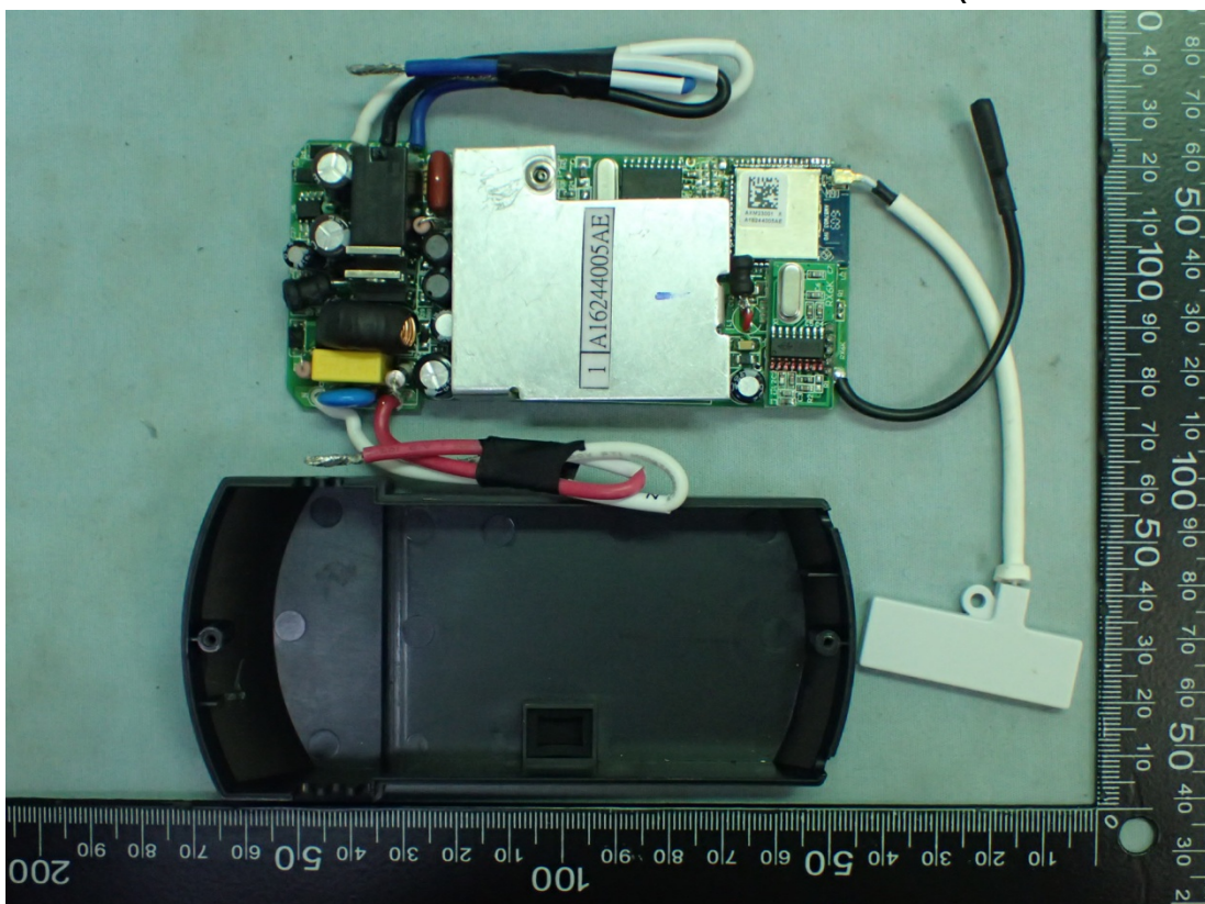
Figure 4 Internal View (Removed Main Board)
