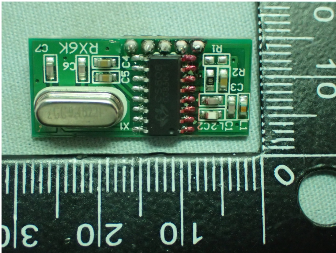
Figure 11 Internal View (RX6K Board, Front View)
