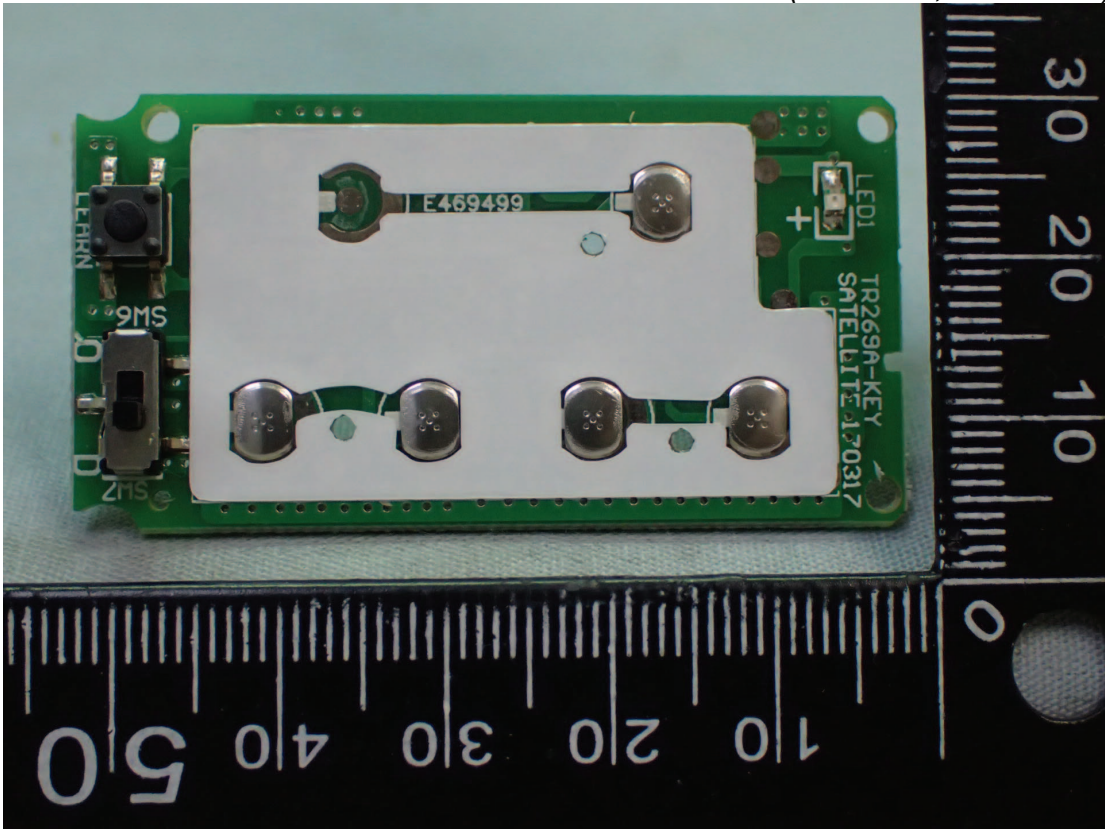
Figure 10 Internal View (RF Board, Back View)
