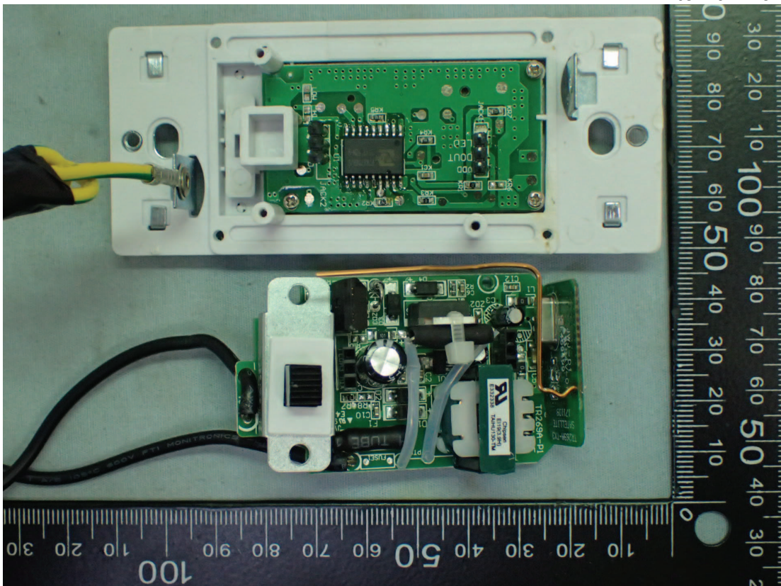
Figure 4 Internal View
