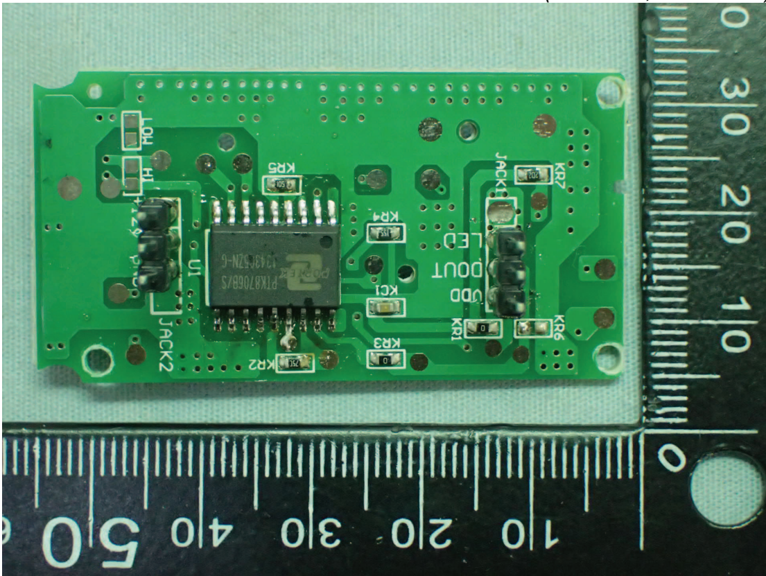
Figure 9 Internal View (RF Board, Front View)
