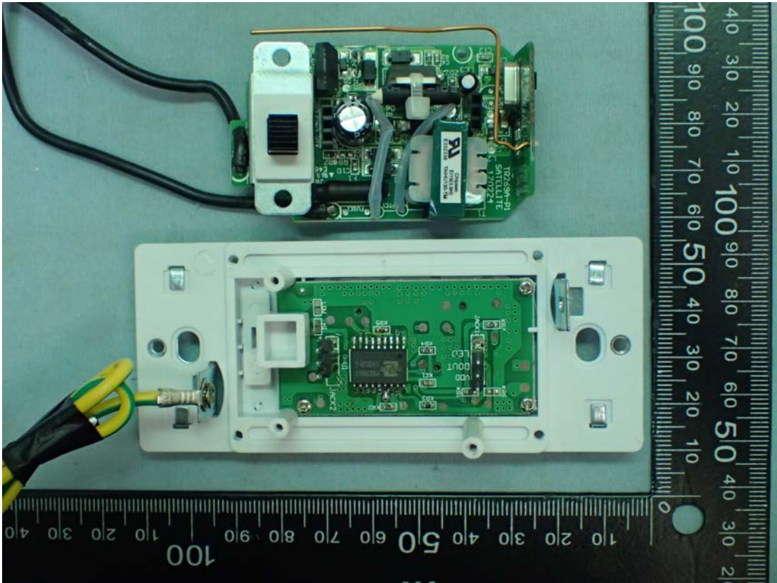
Figure 7 Internal View
