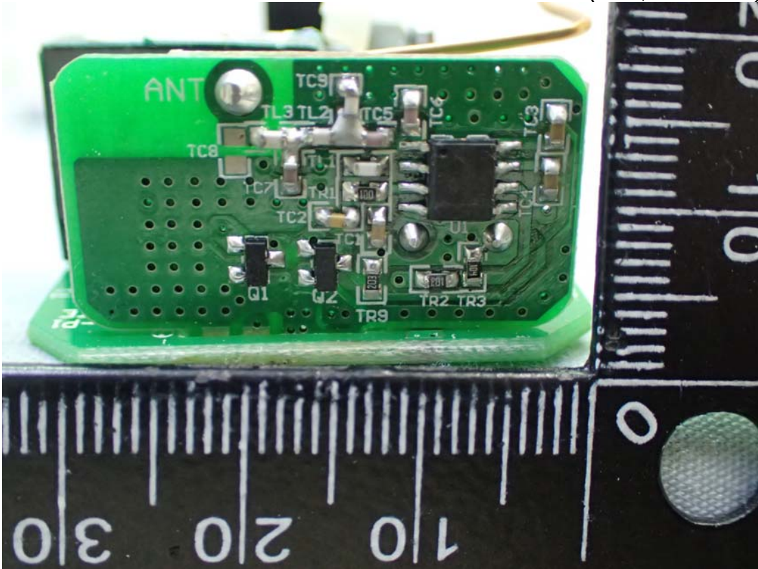
Figure 14 Internal View (PCB, Back View)
