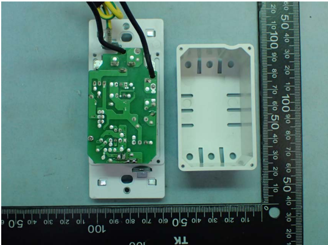
Figure 6 Internal View
