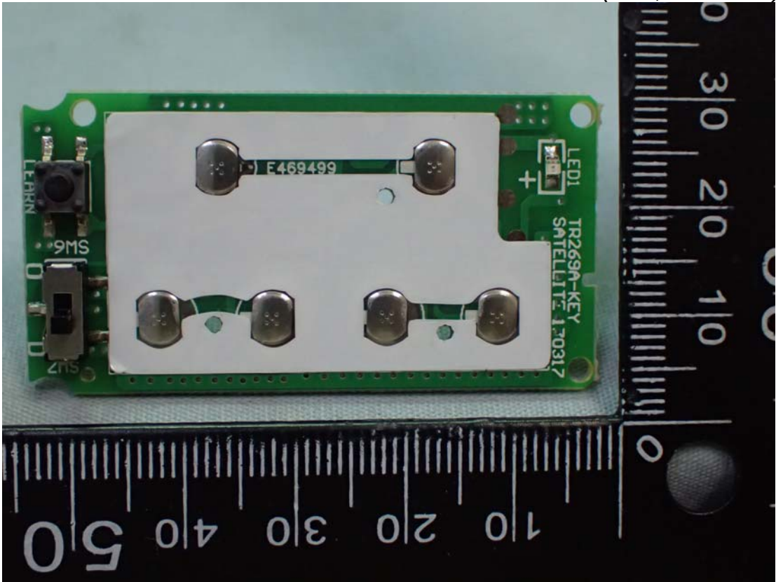
Figure 12 Internal View (PCB, Back View)
