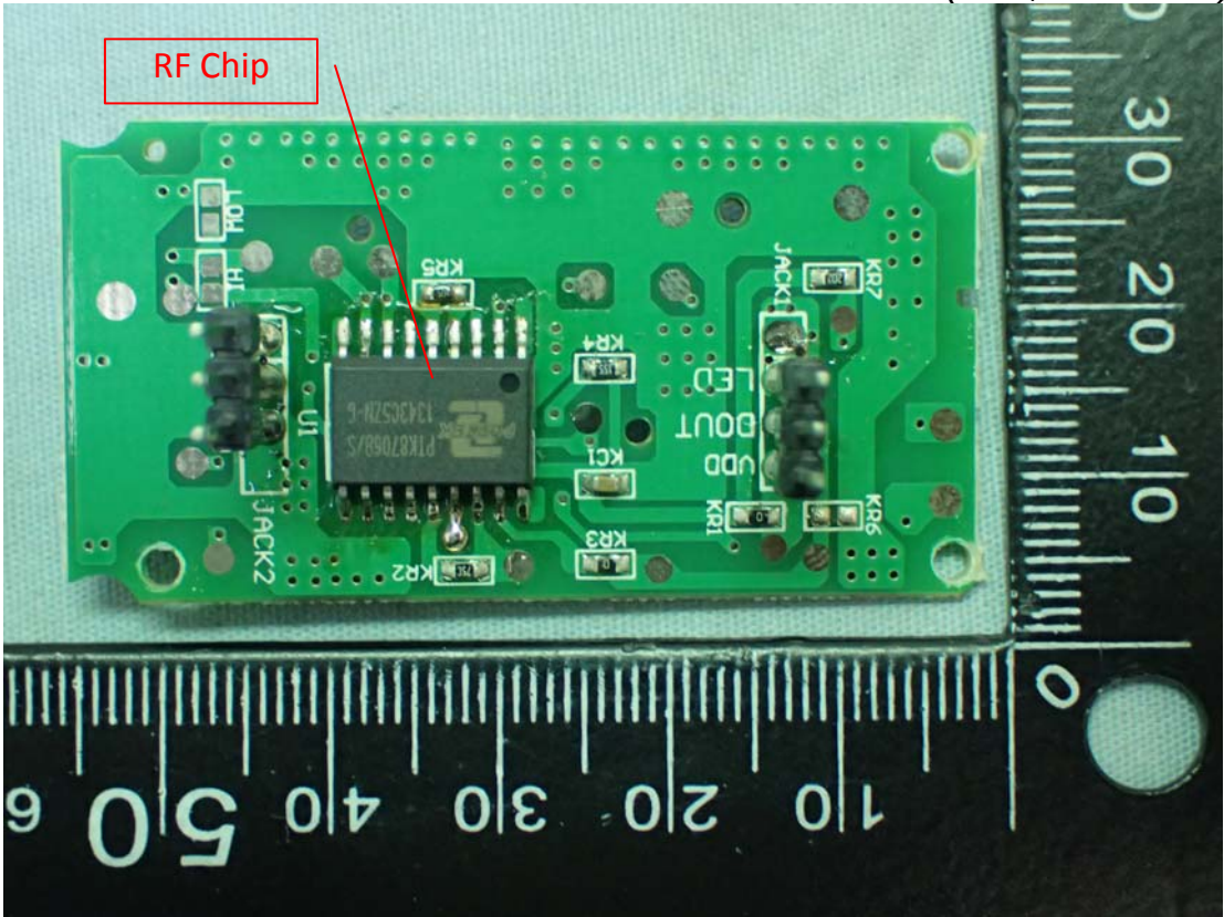
Figure 11 Internal View (PCB, Front View)
