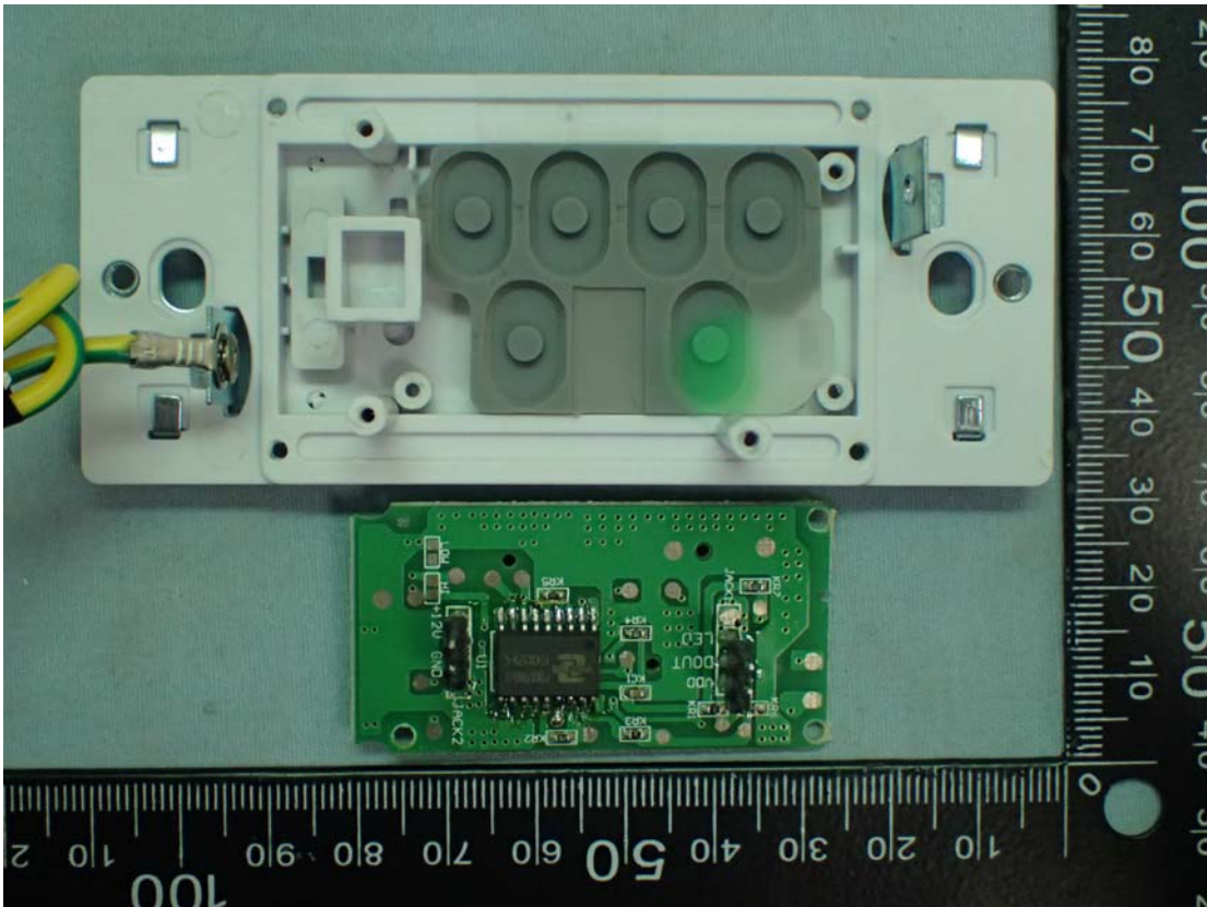
Figure 8 Internal View
