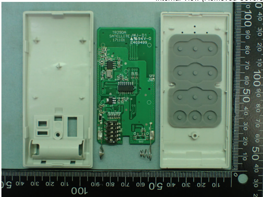
Figure 4 Internal View (Removed Covers)
