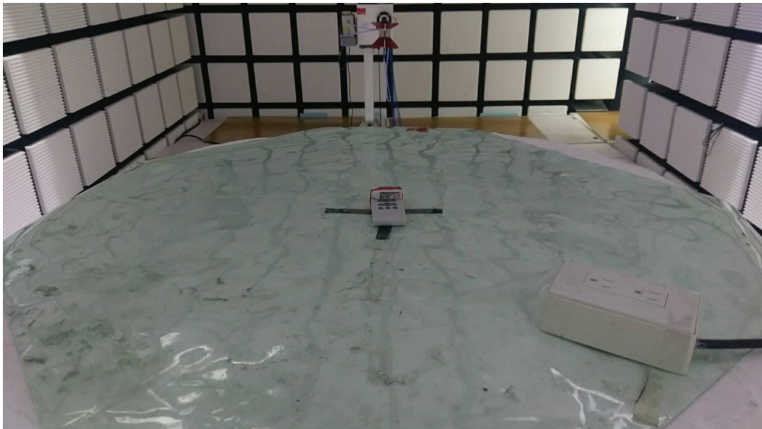
Frequency Range Above 1GHz EUT on Lie
