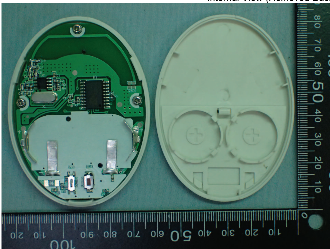
Photo 4 Internal View (Removed Back Cover)
