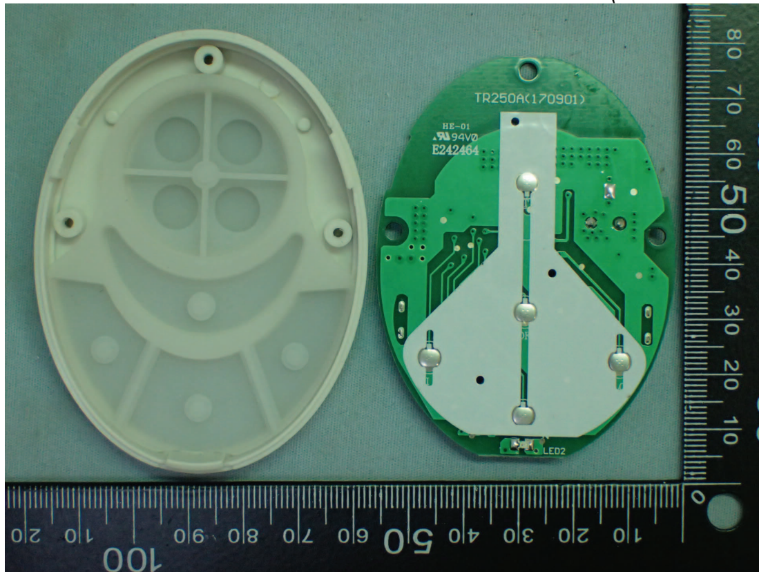
Photo 5 Internal View (Removed Front Cover)
