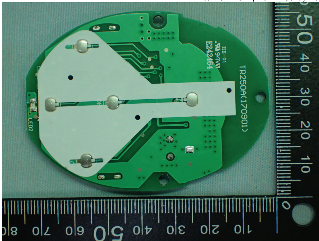
Photo 7 Internal View (Main Board, Back View)
