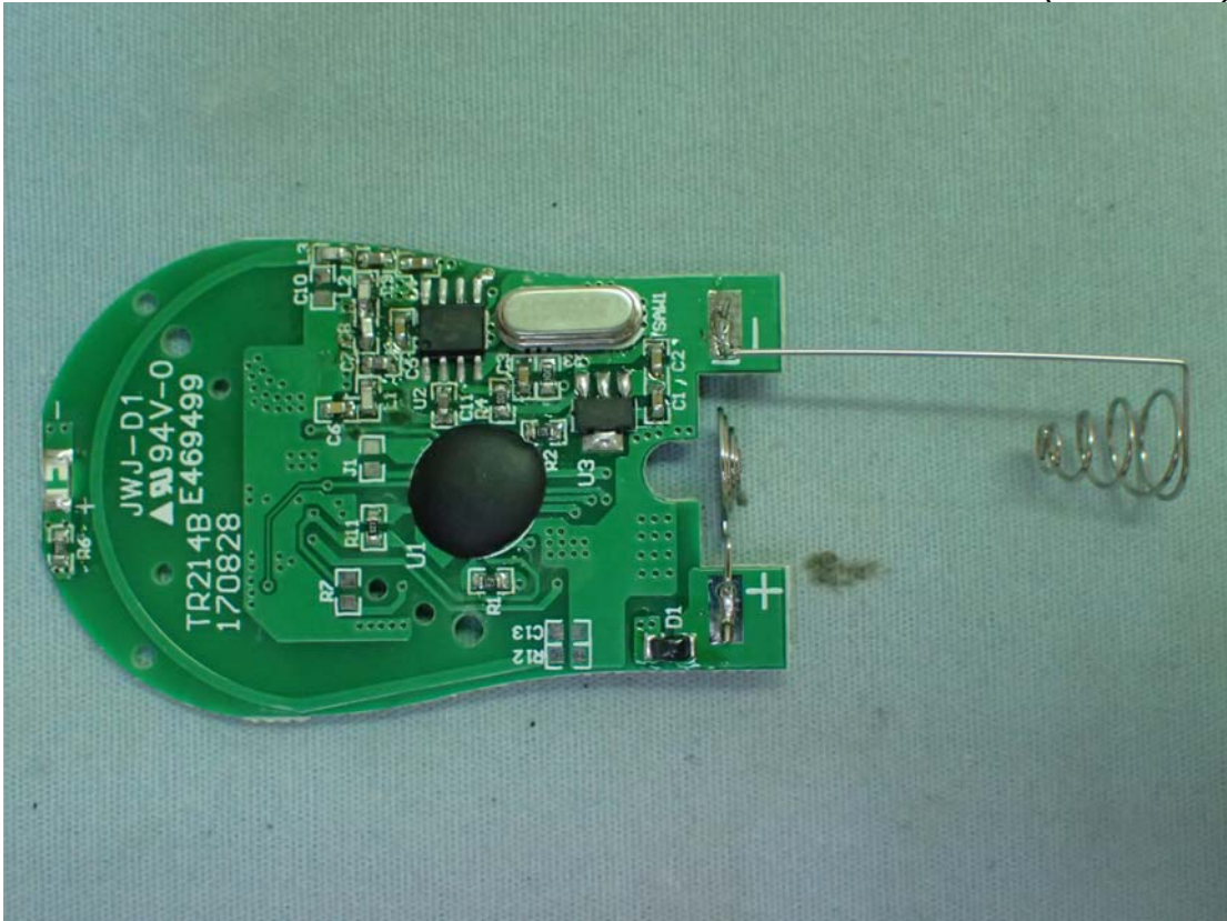
Figure 5 Main Board (Front View)
