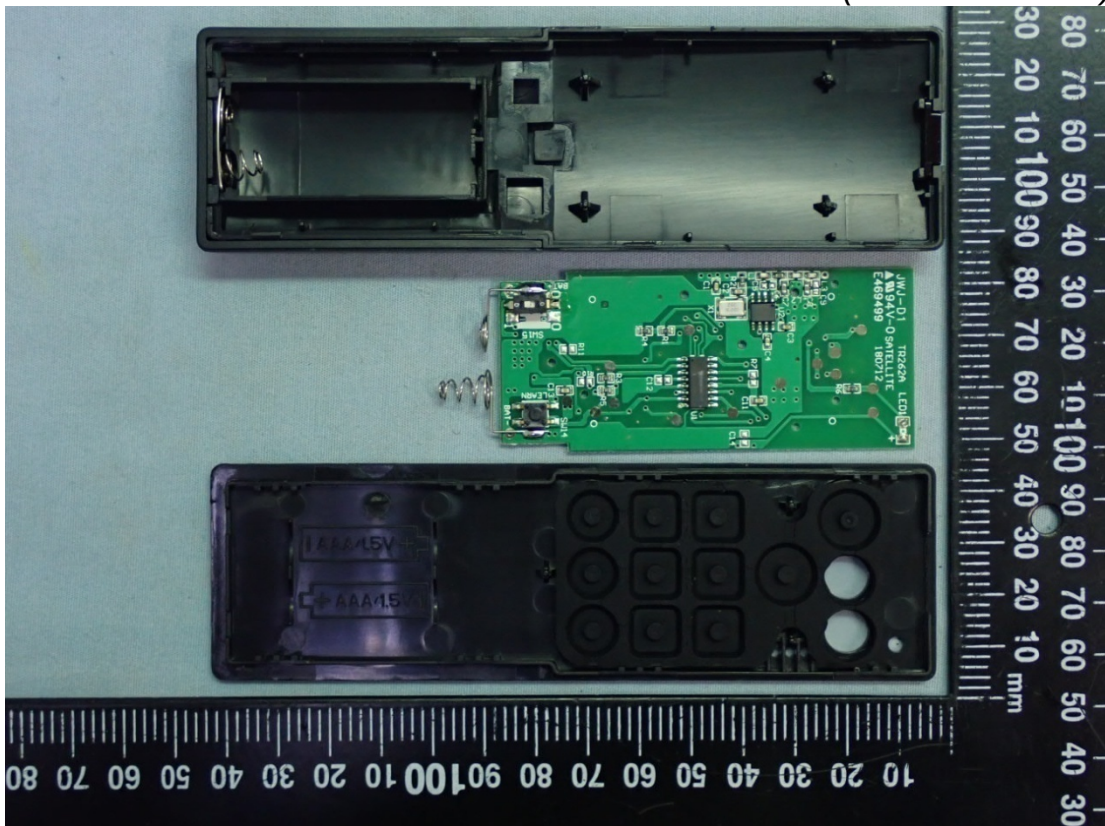
Figure 14 Internal View (Removed Covers)
