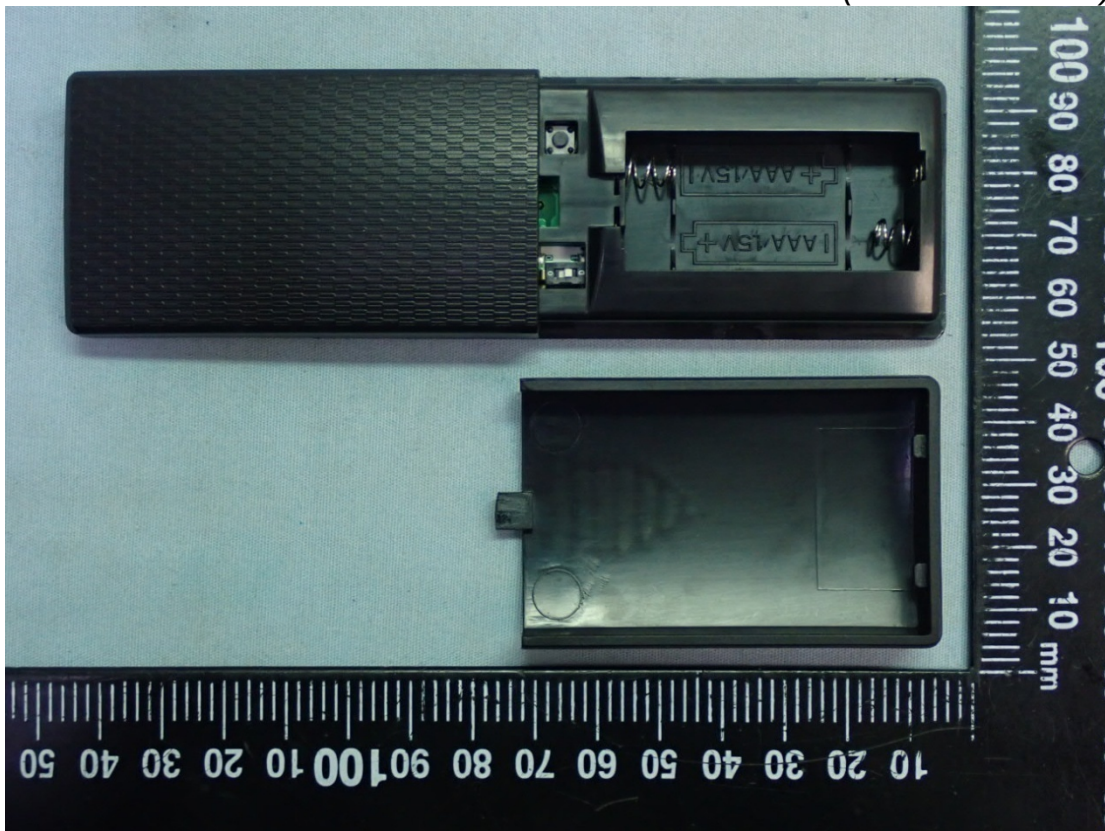
Figure 13 Internal View (Removed Covers)
