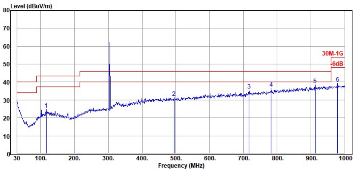
Antenna at Vertical Polarization
