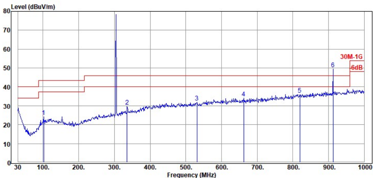
Antenna at Horizontal Polarization
