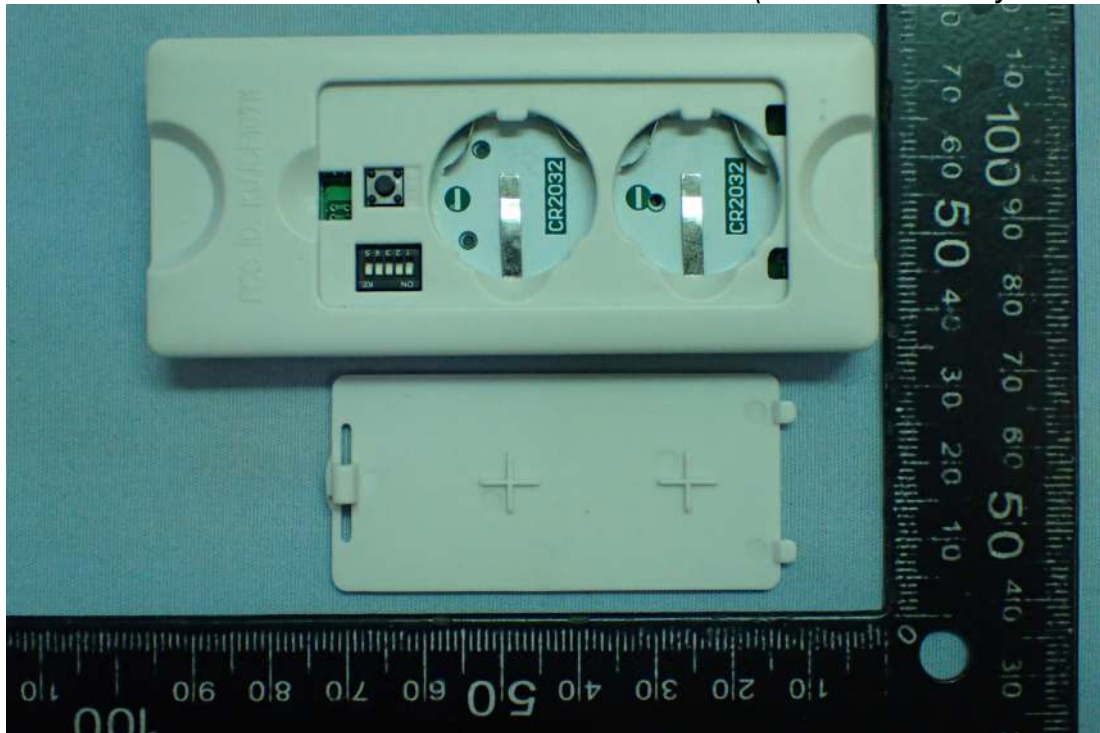
Figure 3 Internal View (Removed Battery Cover)
