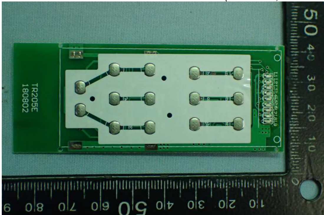
Figure 6 Internal View (Main Board, Back View)
