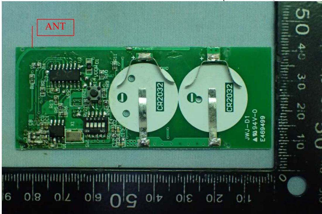
Figure 5 Internal View (Main Board, Front View)
