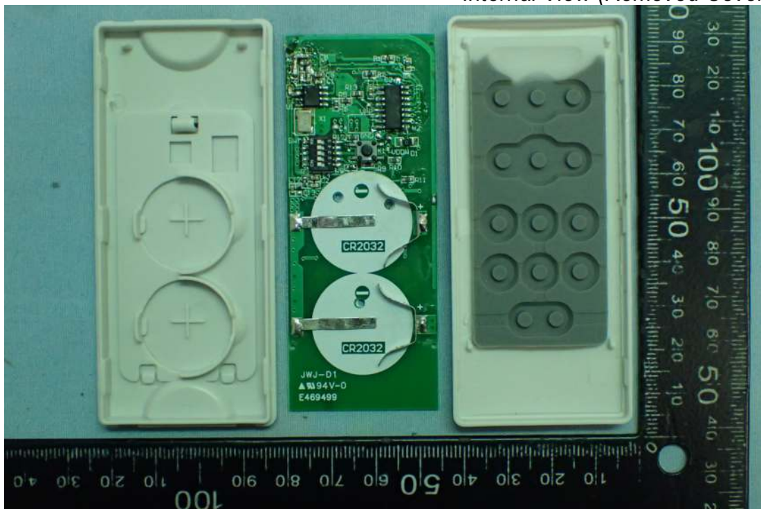
Figure 4 Internal View (Removed Cover)
