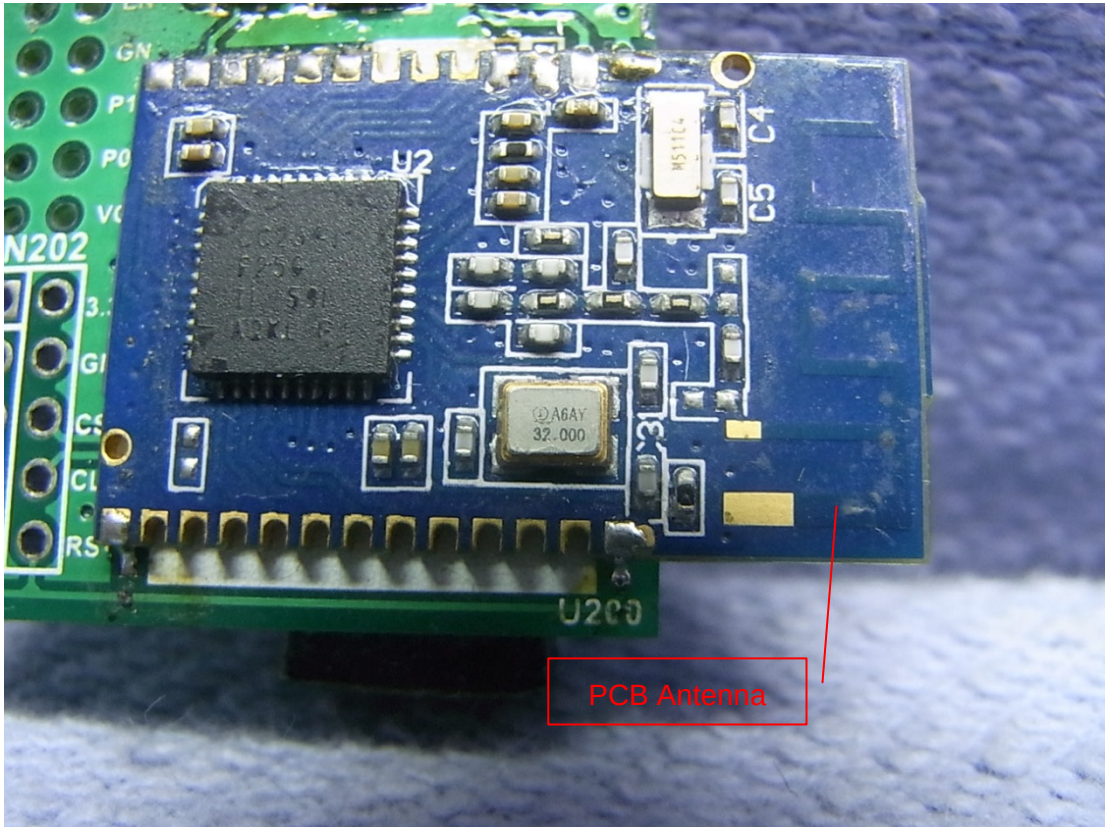
Figure 13 RF Module, Front View
