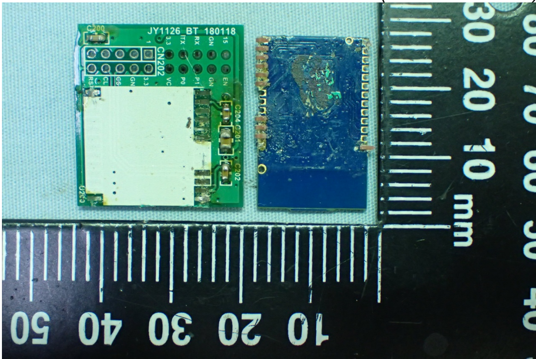
Figure 10 Internal View (Removed RF Module)
