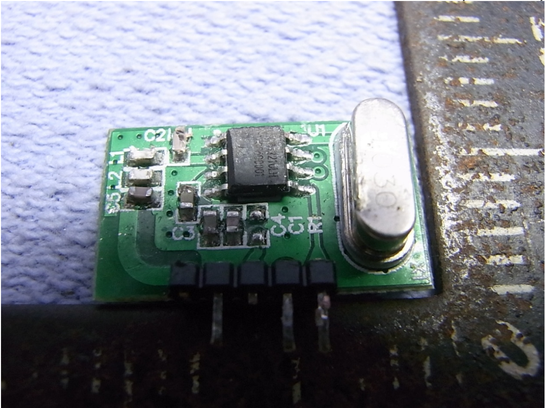
Figure 7 RX module (Front View)
