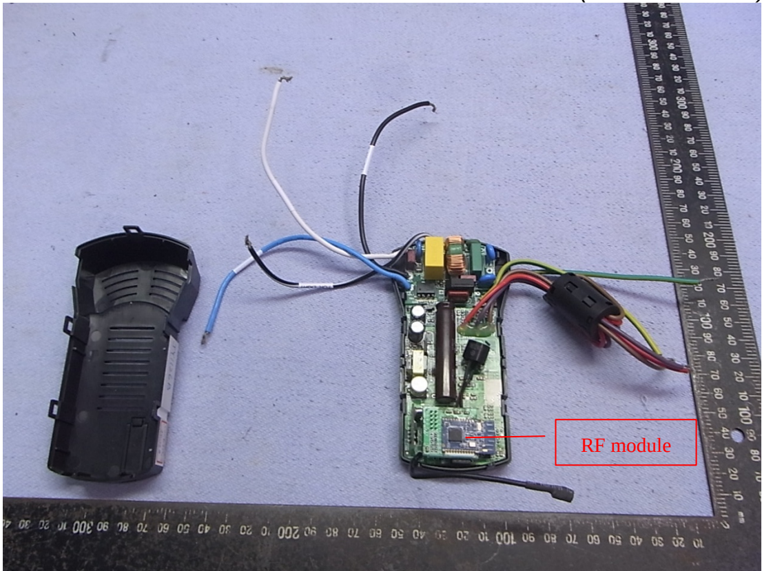
Figure 3 Internal View (Removed Covers)
