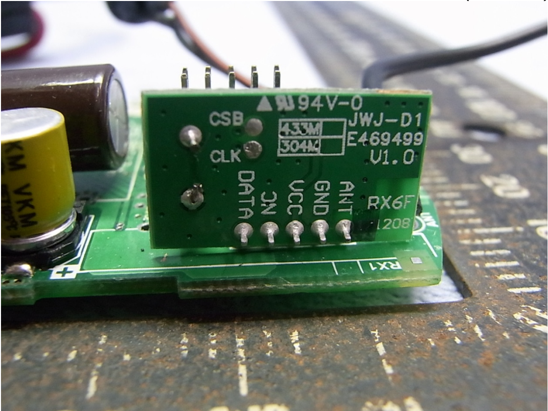
Figure 8 IRX module (Back View)
