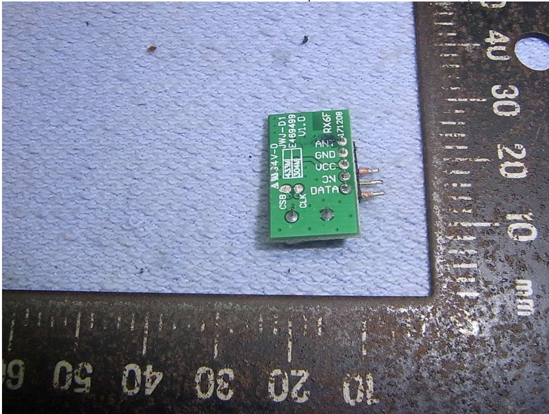
Figure 13 Internal View (RX1 Receiver module, Back View)
