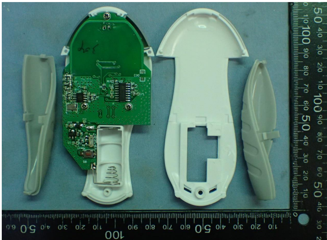
Figure 4 Internal View (Removed Cover)
