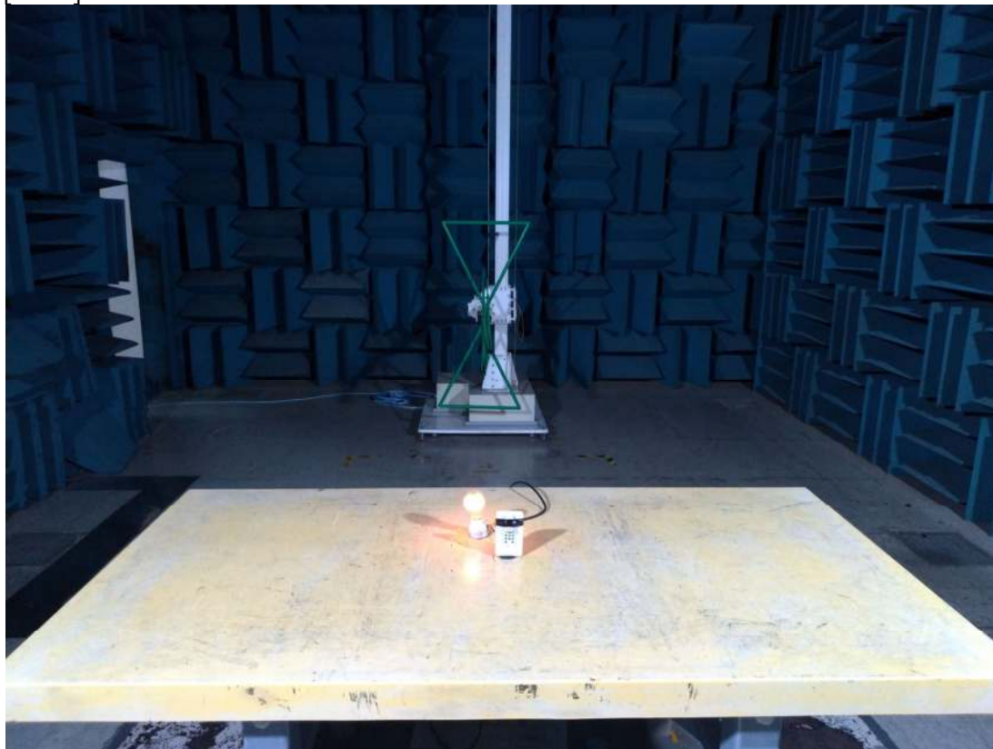
[Stand]
