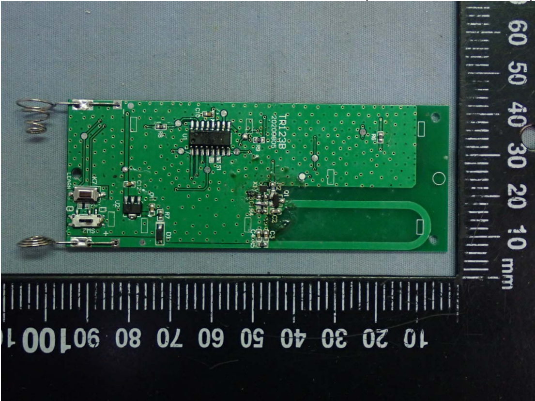
Figure 9 Internal View (Main Board, Front View)
