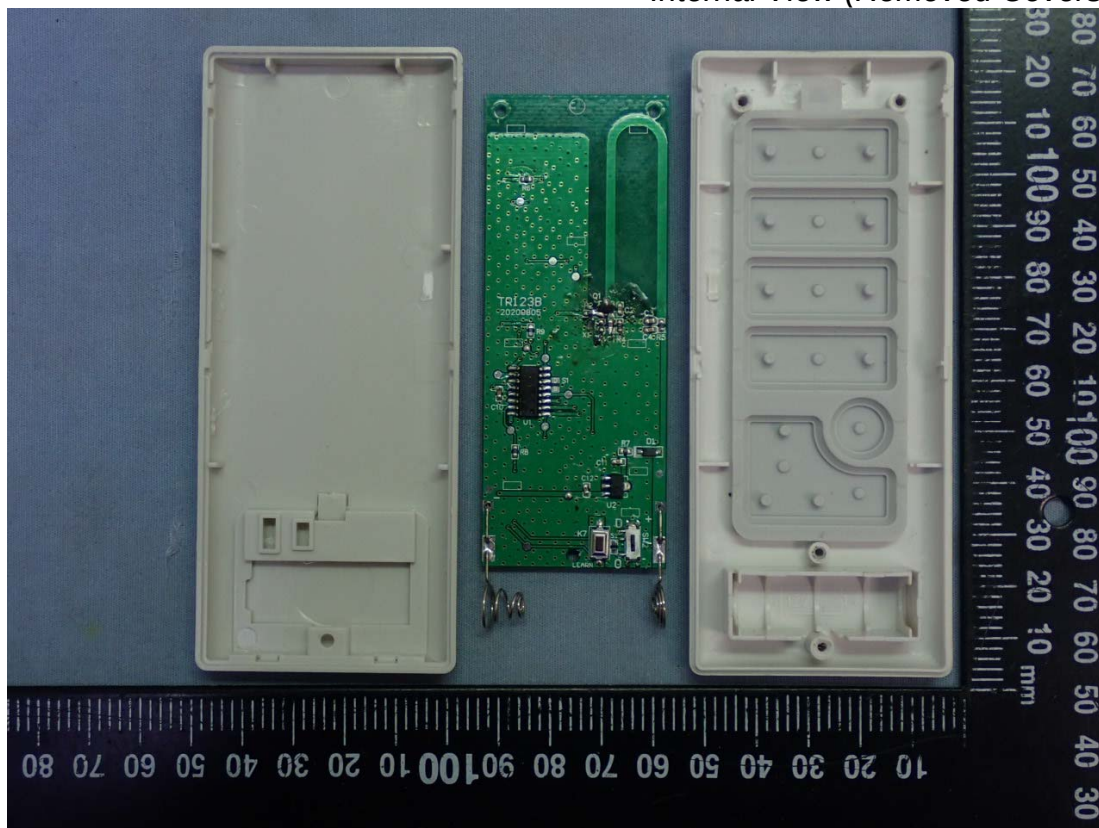
Figure 8 Internal View (Removed Covers)
